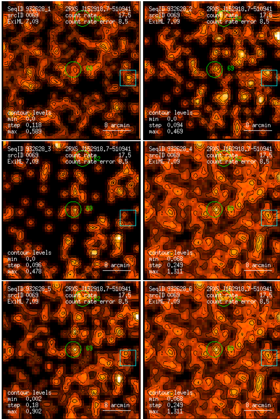
Figure 69: RASS 932628: detection 0069: band rate images, Gaussian filter: (1) PSPC channels 11 – 41, (2) 52 – 90, (3) 91 – 201, (4) 11 – 235, (5) 52 – 201, (6) 11 – 201. Broad band rates in counts/ks. Band rate contour levels in counts/ks/arcmin 2 .
