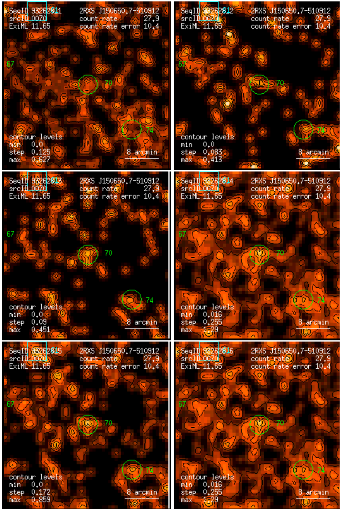
Figure 70: RASS 932628: detection 0070: band rate images, Gaussian filter: (1) PSPC channels 11 – 41, (2) 52 – 90, (3) 91 – 201, (4) 11 – 235, (5) 52 – 201, (6) 11 – 201. Broad band rates in counts/ks. Band rate contour levels in counts/ks/arcmin 2 .
