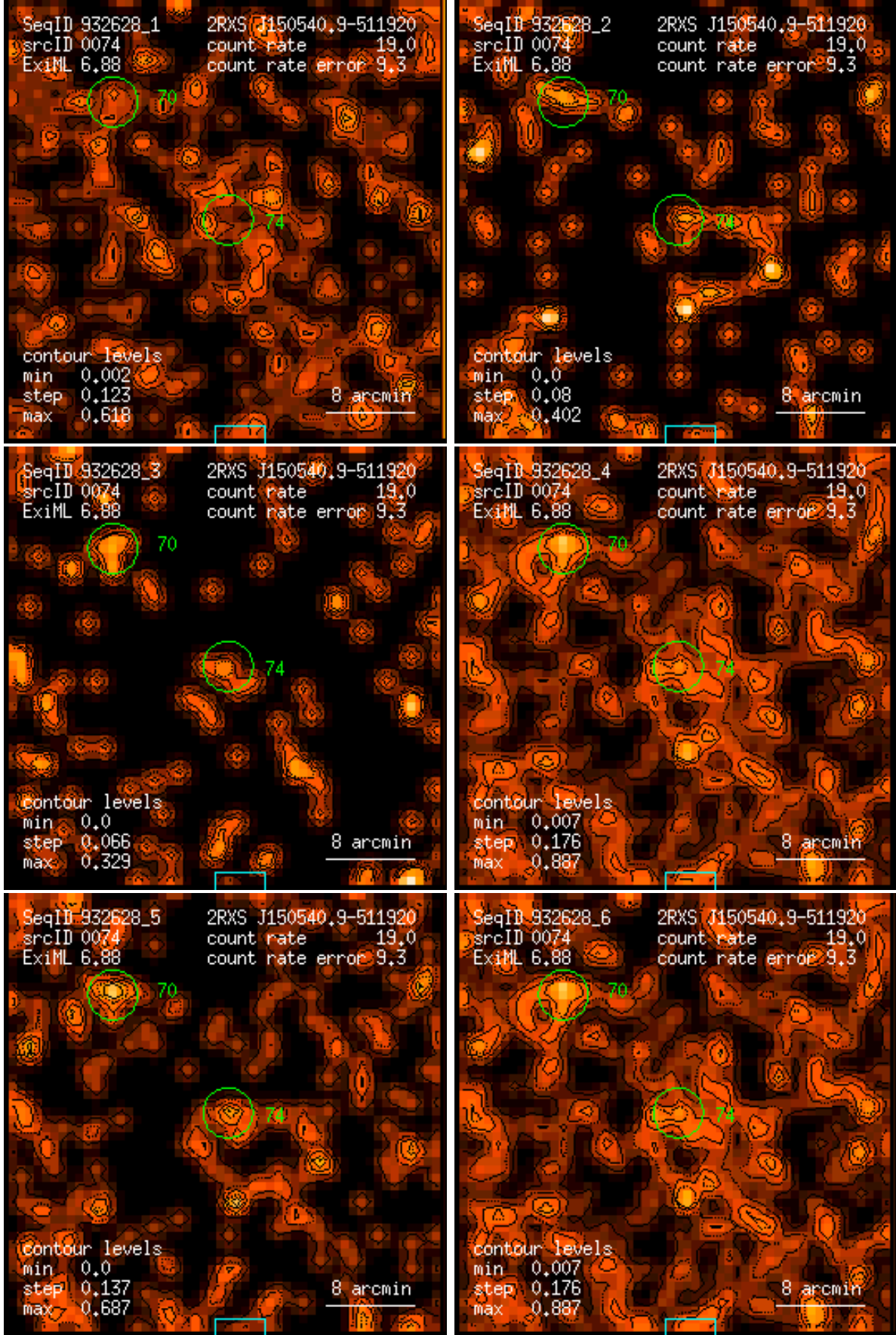
Figure 74: RASS 932628: detection 0074: band rate images, Gaussian filter: (1) PSPC channels 11 – 41, (2) 52 – 90, (3) 91 – 201, (4) 11 – 235, (5) 52 – 201, (6) 11 – 201. Broad band rates in counts/ks. Band rate contour levels in counts/ks/arcmin 2 .
