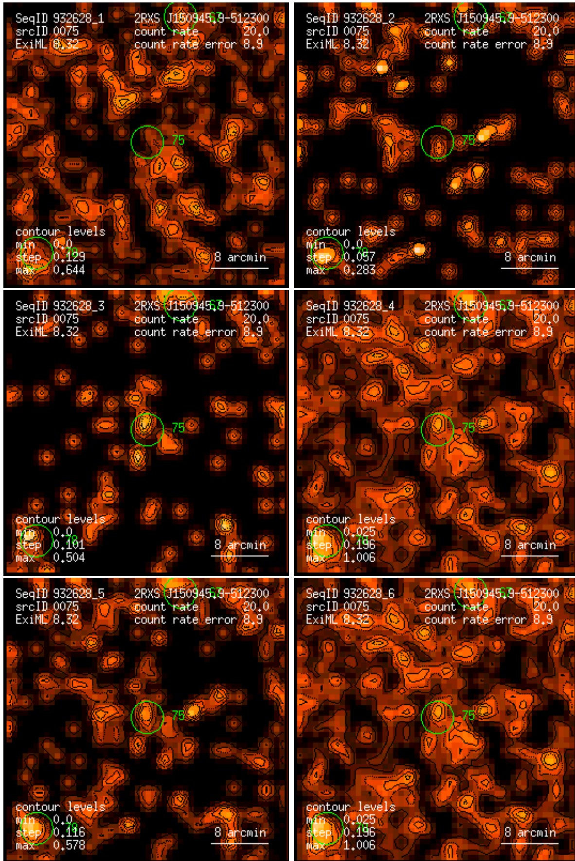
Figure 75: RASS 932628: detection 0075: band rate images, Gaussian filter: (1) PSPC channels 11 – 41, (2) 52 – 90, (3) 91 – 201, (4) 11 – 235, (5) 52 – 201, (6) 11 – 201. Broad band rates in counts/ks. Band rate contour levels in counts/ks/arcmin 2 .
