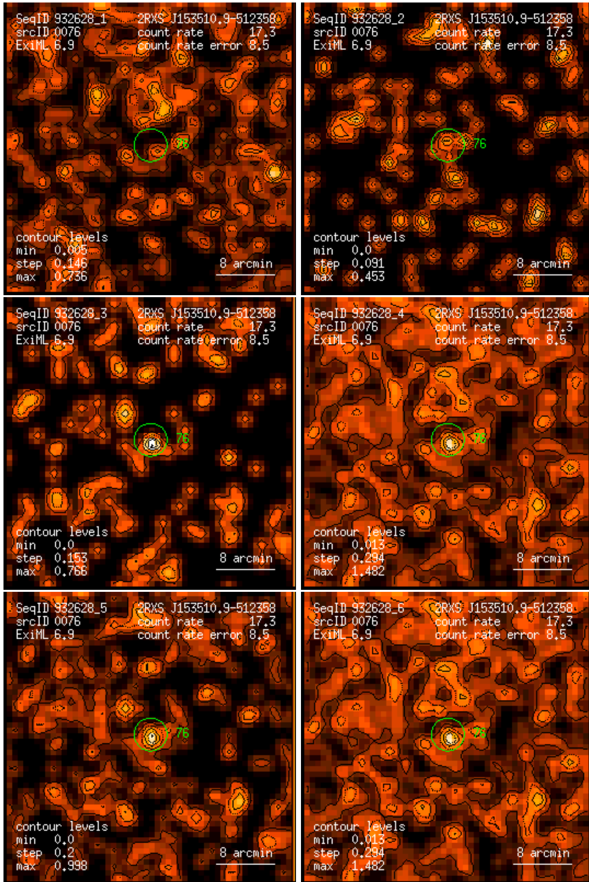
Figure 76: RASS 932628: detection 0076: band rate images, Gaussian filter: (1) PSPC channels 11 – 41, (2) 52 – 90, (3) 91 – 201, (4) 11 – 235, (5) 52 – 201, (6) 11 – 201. Broad band rates in counts/ks. Band rate contour levels in counts/ks/arcmin 2 .
