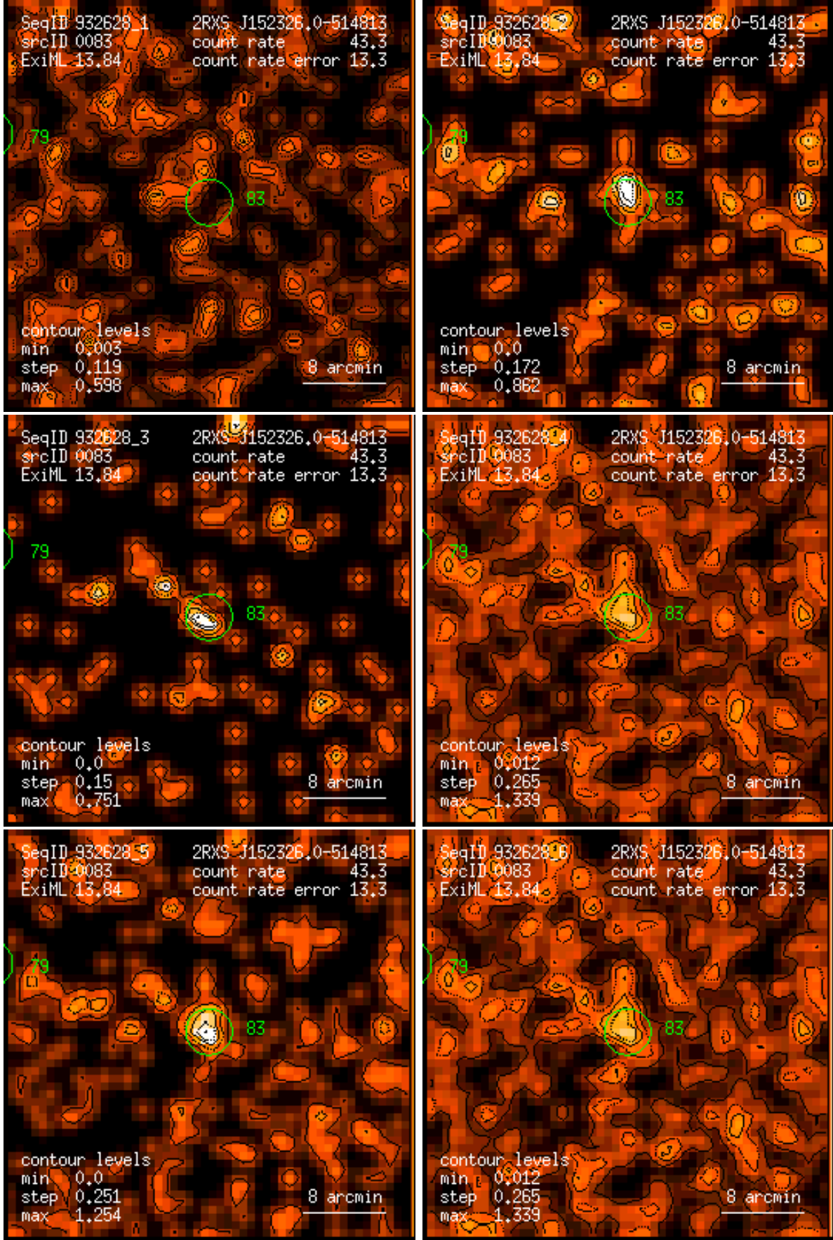
Figure 83: RASS 932628: detection 0083: band rate images, Gaussian filter: (1) PSPC channels 11 – 41, (2) 52 – 90, (3) 91 – 201, (4) 11 – 235, (5) 52 – 201, (6) 11 – 201. Broad band rates in counts/ks. Band rate contour levels in counts/ks/arcmin 2 .
