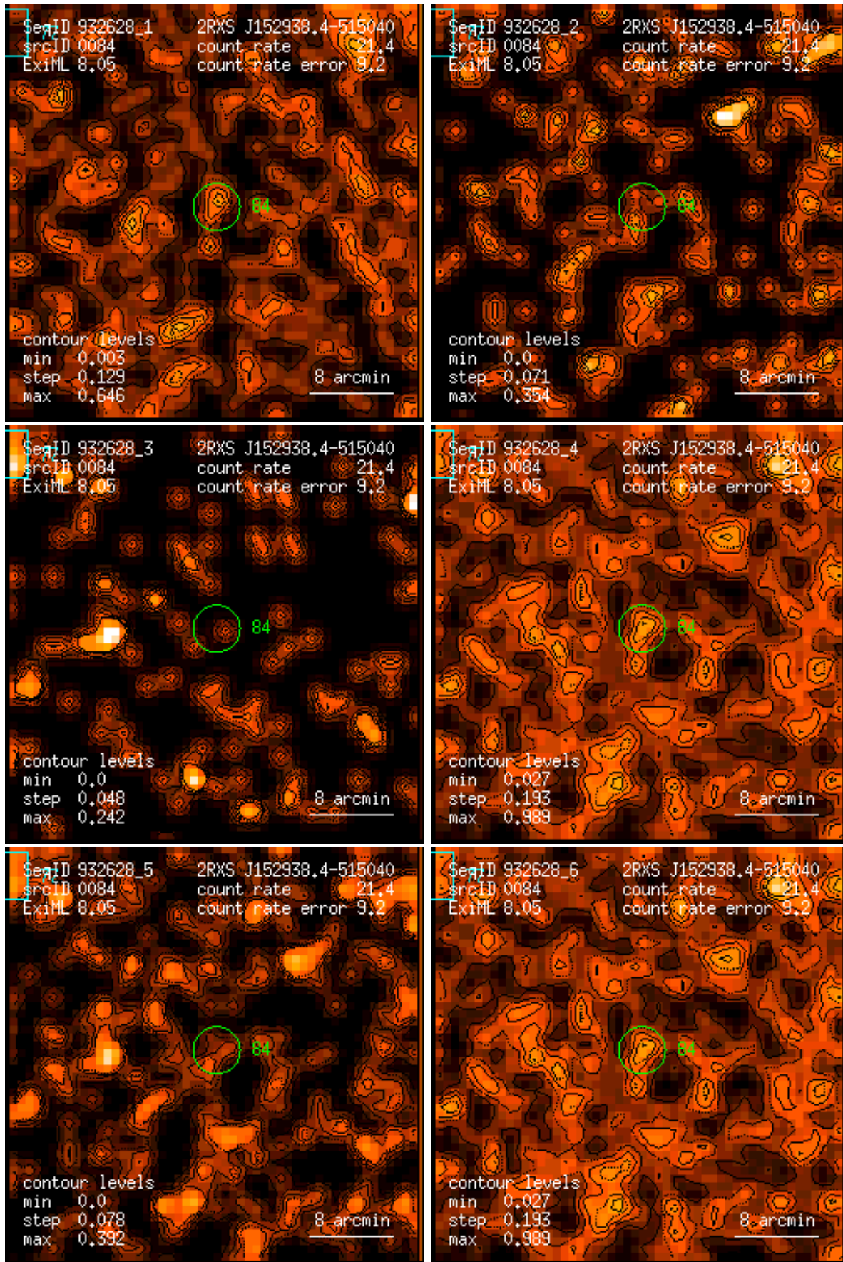
Figure 84: RASS 932628: detection 0084: band rate images, Gaussian filter: (1) PSPC channels 11 – 41, (2) 52 – 90, (3) 91 – 201, (4) 11 – 235, (5) 52 – 201, (6) 11 – 201. Broad band rates in counts/ks. Band rate contour levels in counts/ks/arcmin 2 .
