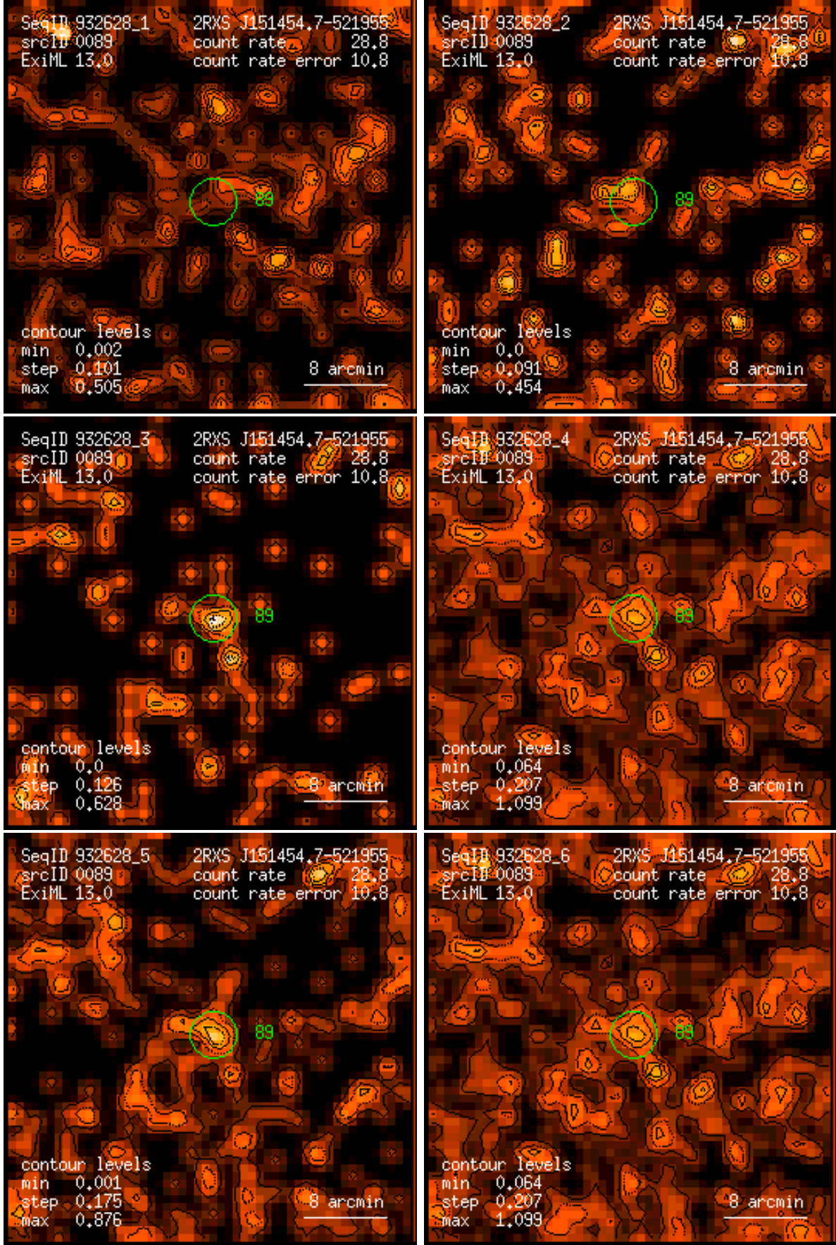
Figure 89: RASS 932628: detection 0089: band rate images, Gaussian filter: (1) PSPC channels 11 – 41, (2) 52 – 90, (3) 91 – 201, (4) 11 – 235, (5) 52 – 201, (6) 11 – 201. Broad band rates in counts/ks. Band rate contour levels in counts/ks/arcmin 2 .
