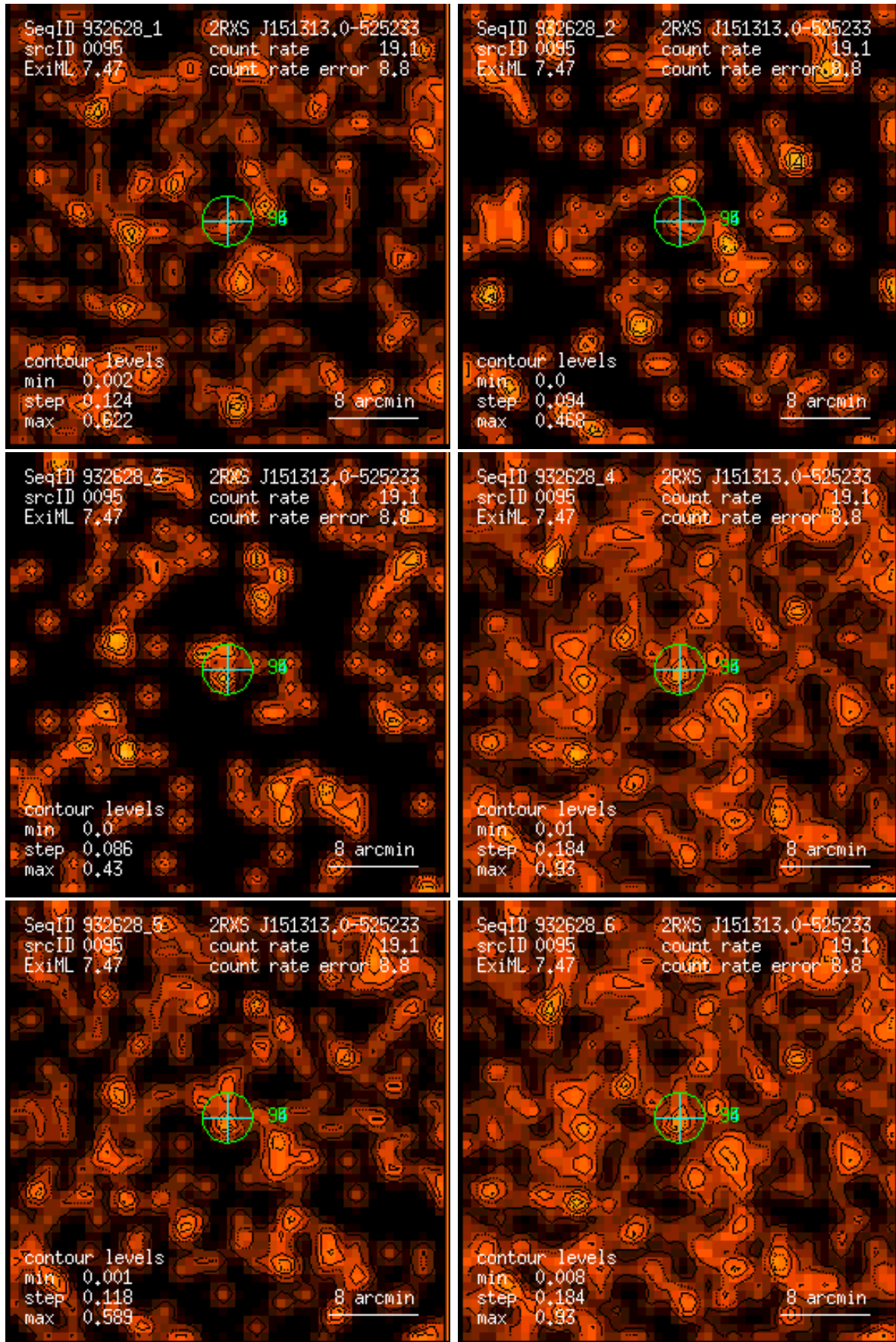
Figure 95: RASS 932628: detection 0095: band rate images, Gaussian filter: (1) PSPC channels 11 – 41, (2) 52 – 90, (3) 91 – 201, (4) 11 – 235, (5) 52 – 201, (6) 11 – 201. Broad band rates in counts/ks. Band rate contour levels in counts/ks/arcmin 2 .
