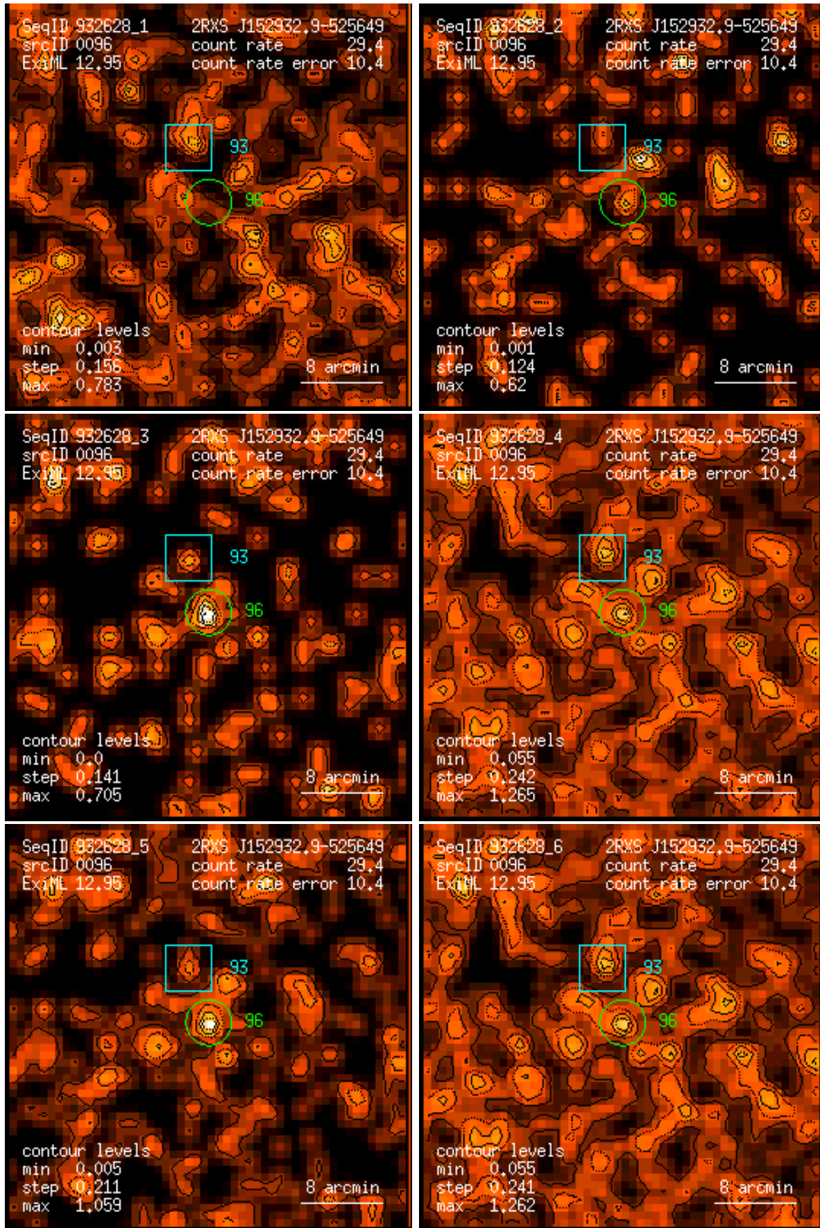
Figure 96: RASS 932628: detection 0096: band rate images, Gaussian filter: (1) PSPC channels 11 – 41, (2) 52 – 90, (3) 91 – 201, (4) 11 – 235, (5) 52 – 201, (6) 11 – 201. Broad band rates in counts/ks. Band rate contour levels in counts/ks/arcmin 2 .
