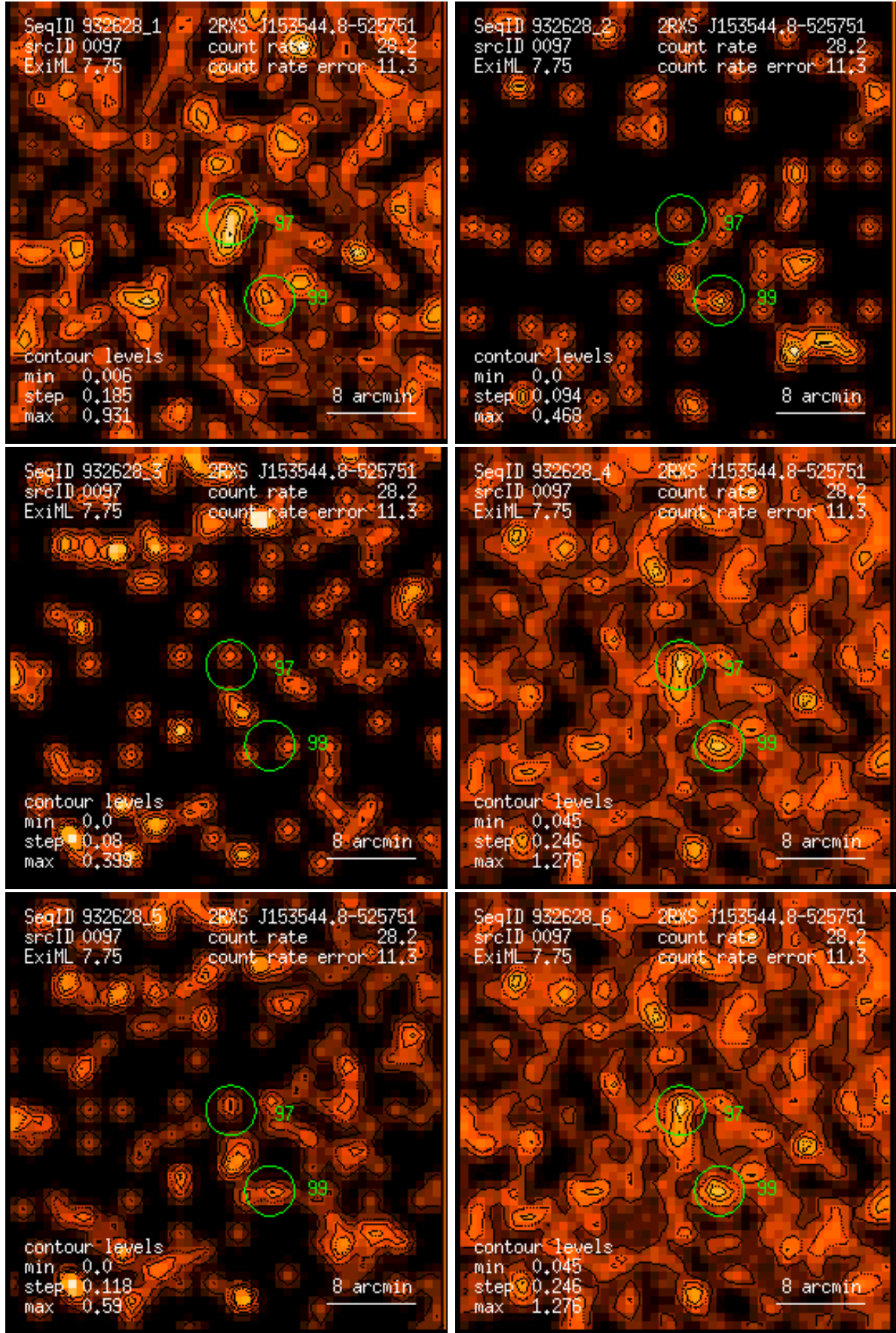
Figure 97: RASS 932628: detection 0097: band rate images, Gaussian filter: (1) PSPC channels 11 – 41, (2) 52 – 90, (3) 91 – 201, (4) 11 – 235, (5) 52 – 201, (6) 11 – 201. Broad band rates in counts/ks. Band rate contour levels in counts/ks/arcmin 2 .
