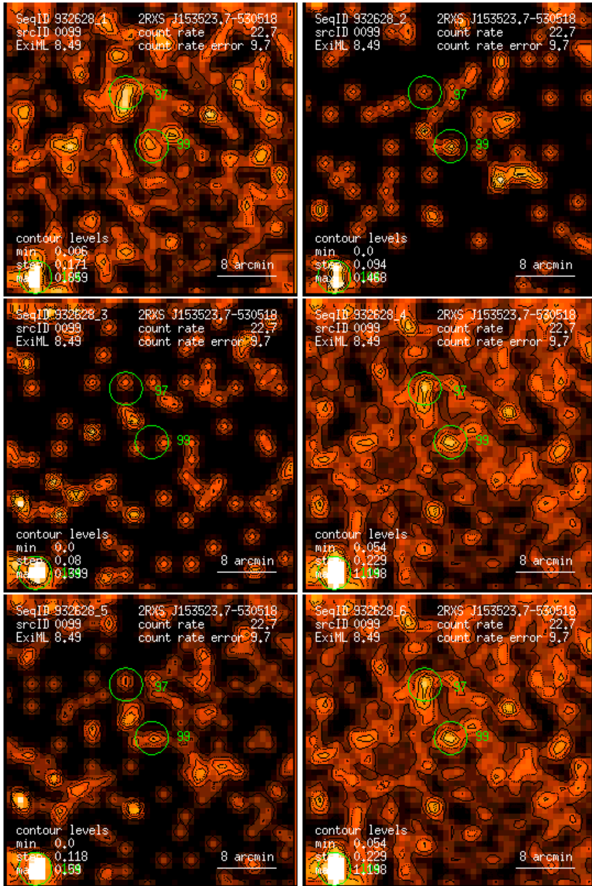
Figure 99: RASS 932628: detection 0099: band rate images, Gaussian filter: (1) PSPC channels 11 – 41, (2) 52 – 90, (3) 91 – 201, (4) 11 – 235, (5) 52 – 201, (6) 11 – 201. Broad band rates in counts/ks. Band rate contour levels in counts/ks/arcmin 2 .
