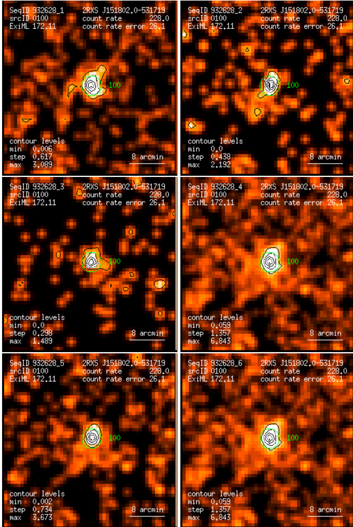
Figure 100: RASS 932628: detection 0100: band rate images, Gaussian filter: (1) PSPC channels 11 – 41, (2) 52 – 90, (3) 91 – 201, (4) 11 – 235, (5) 52 – 201, (6) 11 – 201. Broad band rates in counts/ks. Band rate contour levels in counts/ks/arcmin 2 .
