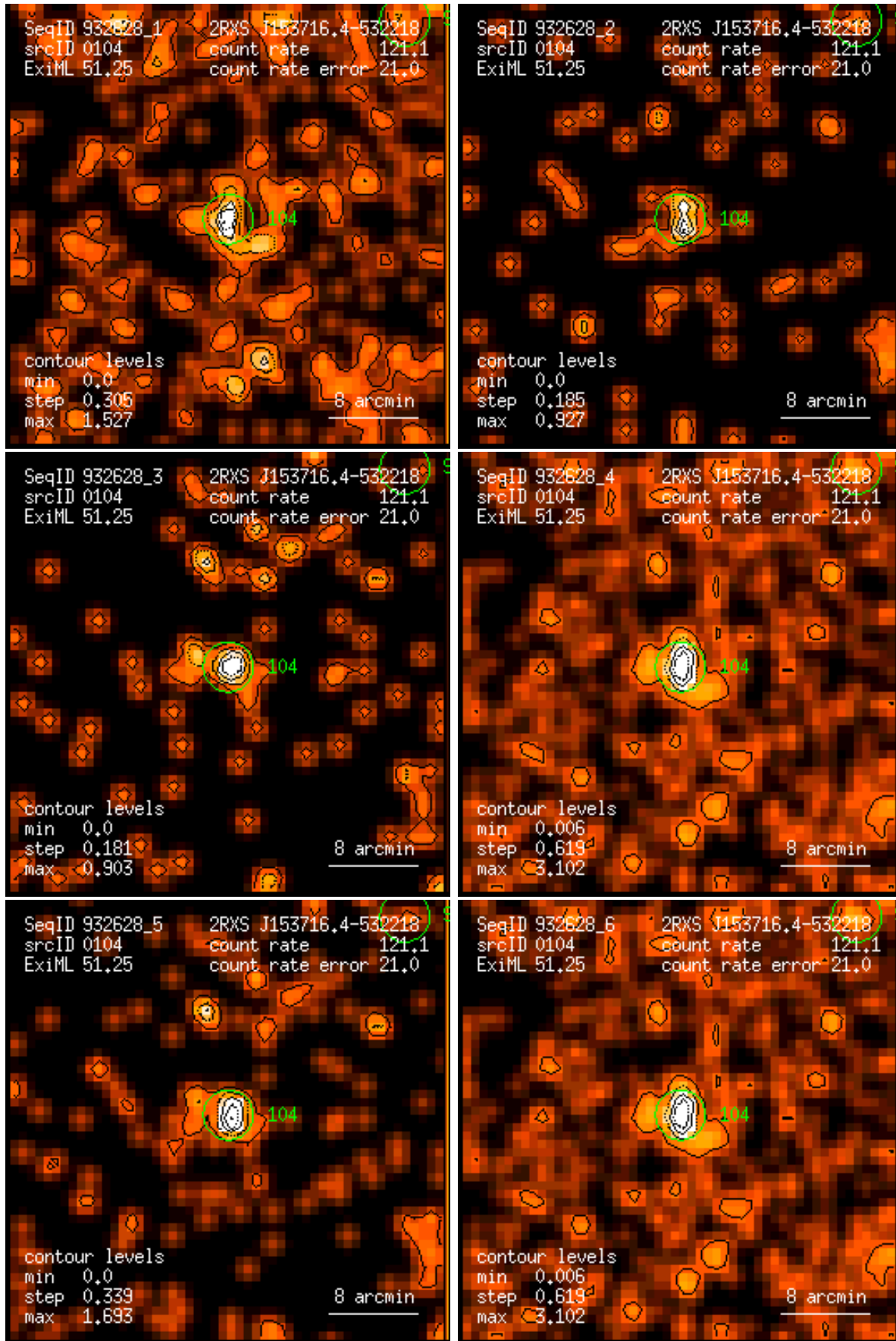
Figure 104: RASS 932628: detection 0104: band rate images, Gaussian filter: (1) PSPC channels 11 – 41, (2) 52 – 90, (3) 91 – 201, (4) 11 – 235, (5) 52 – 201, (6) 11 – 201. Broad band rates in counts/ks. Band rate contour levels in counts/ks/arcmin 2 .
