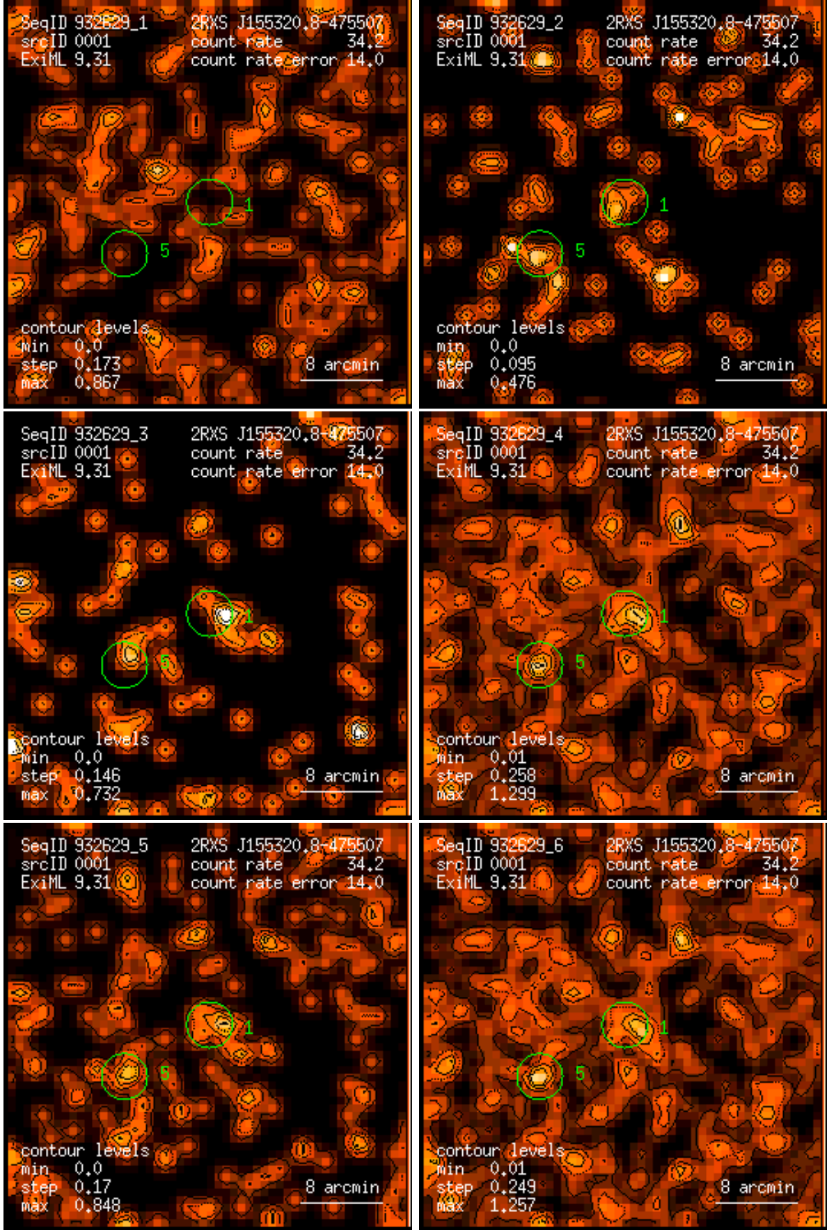
Figure 1: RASS 932629: detection 0001: band rate images, Gaussian filter: (1) PSPC channels 11 – 41, (2) 52 – 90, (3) 91 – 201, (4) 11 – 235, (5) 52 – 201, (6) 11 – 201. Broad band rates in counts/ks. Band rate contour levels in counts/ks/arcmin 2 .
