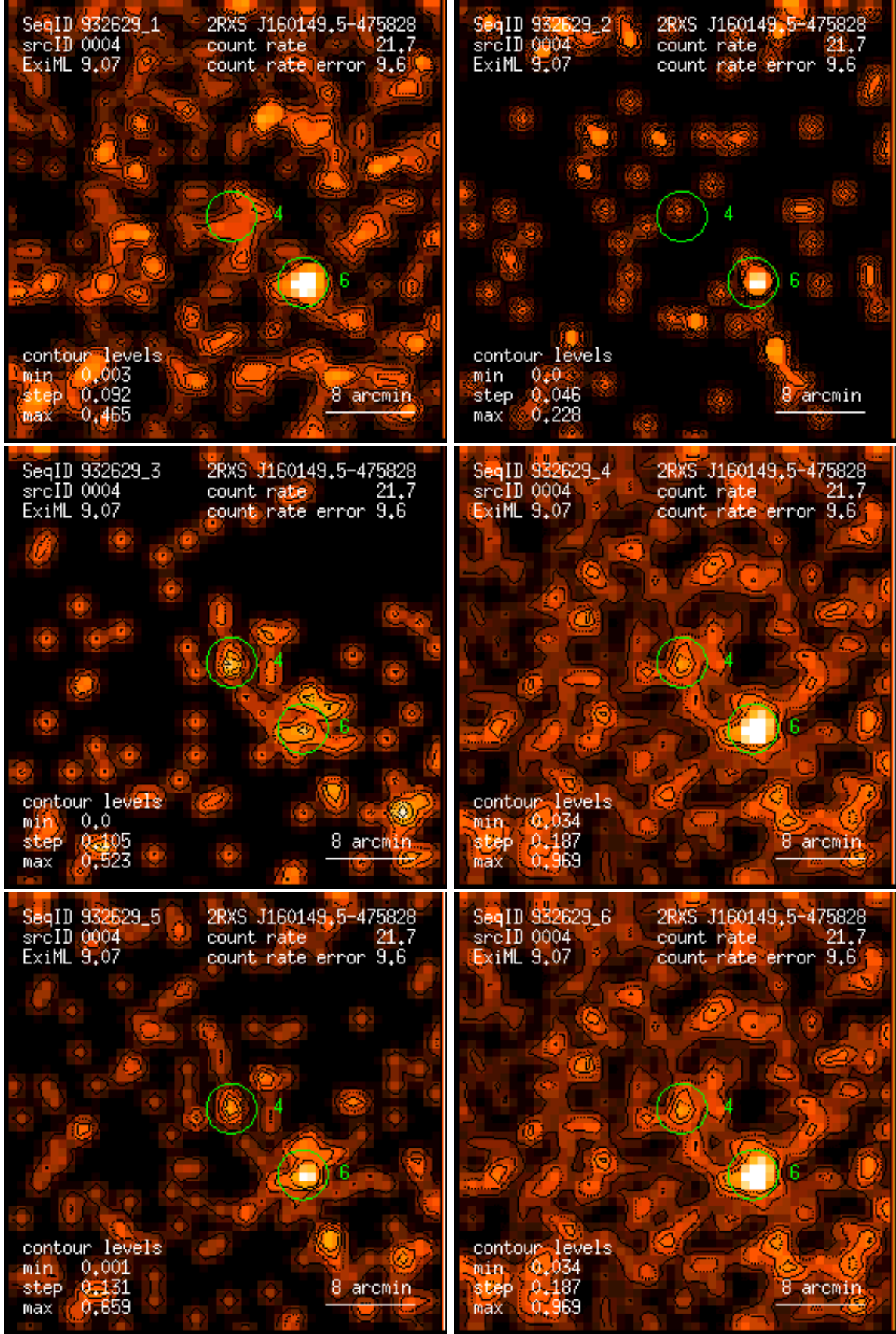
Figure 4: RASS 932629: detection 0004: band rate images, Gaussian filter: (1) PSPC channels 11 – 41, (2) 52 – 90, (3) 91 – 201, (4) 11 – 235, (5) 52 – 201, (6) 11 – 201. Broad band rates in counts/ks. Band rate contour levels in counts/ks/arcmin 2 .
