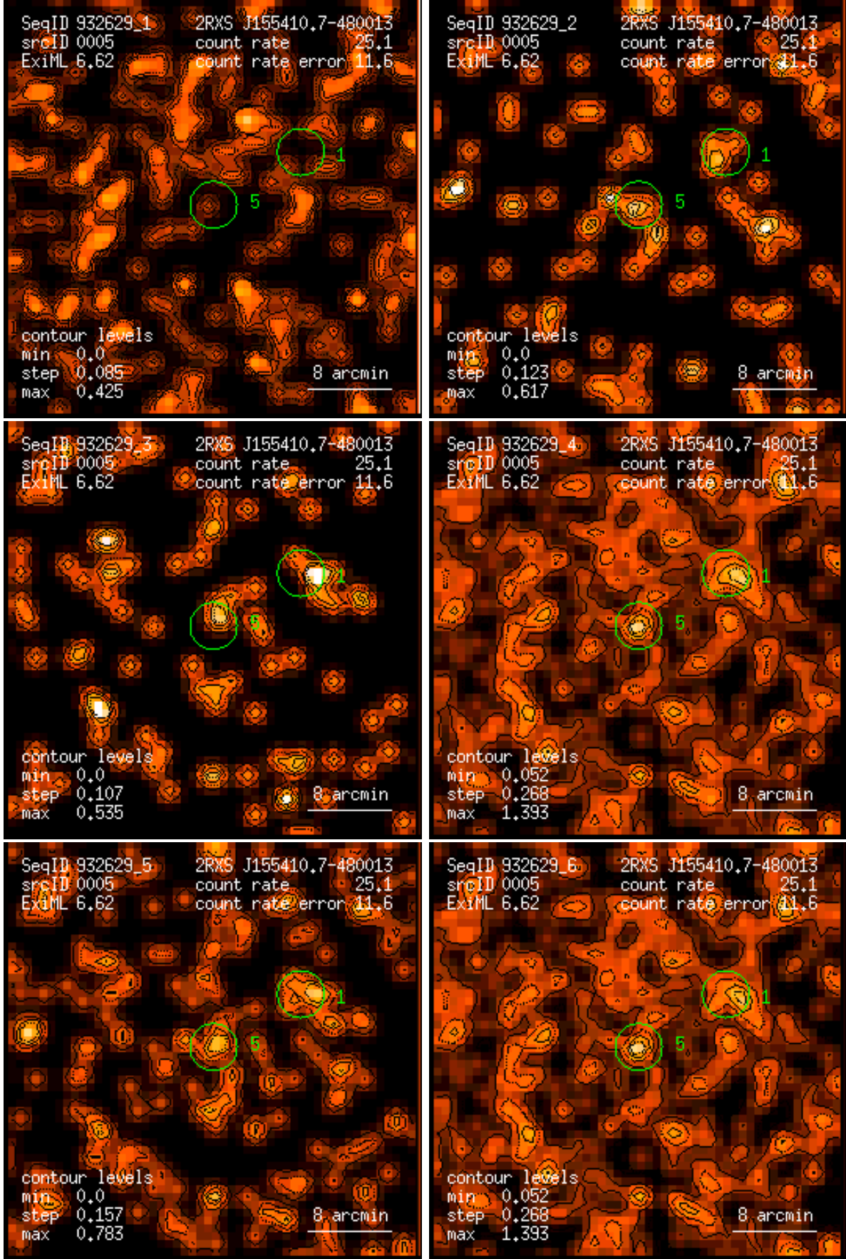
Figure 5: RASS 932629: detection 0005: band rate images, Gaussian filter: (1) PSPC channels 11 – 41, (2) 52 – 90, (3) 91 – 201, (4) 11 – 235, (5) 52 – 201, (6) 11 – 201. Broad band rates in counts/ks. Band rate contour levels in counts/ks/arcmin 2 .
