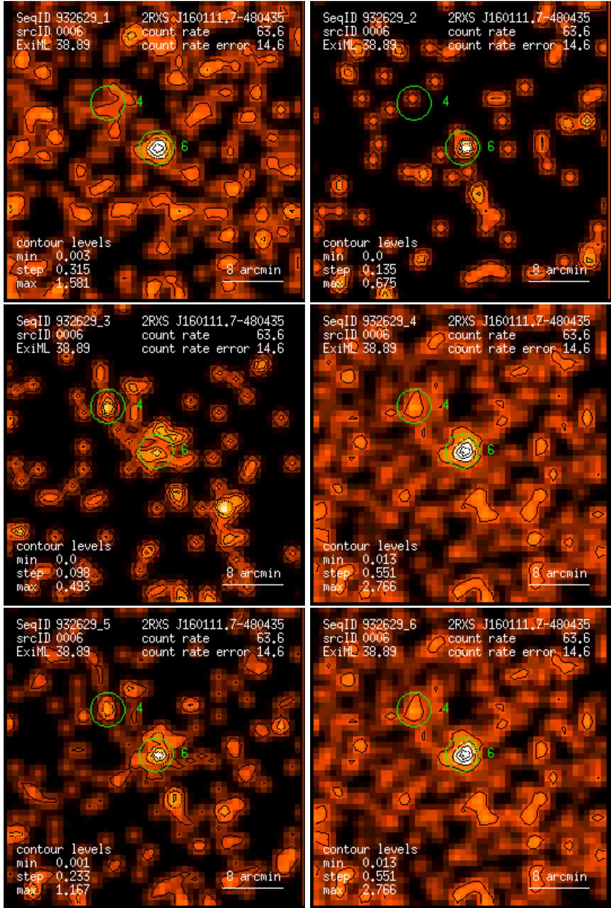
Figure 6: RASS 932629: detection 0006: band rate images, Gaussian filter: (1) PSPC channels 11 – 41, (2) 52 – 90, (3) 91 – 201, (4) 11 – 235, (5) 52 – 201, (6) 11 – 201. Broad band rates in counts/ks. Band rate contour levels in counts/ks/arcmin 2 .
