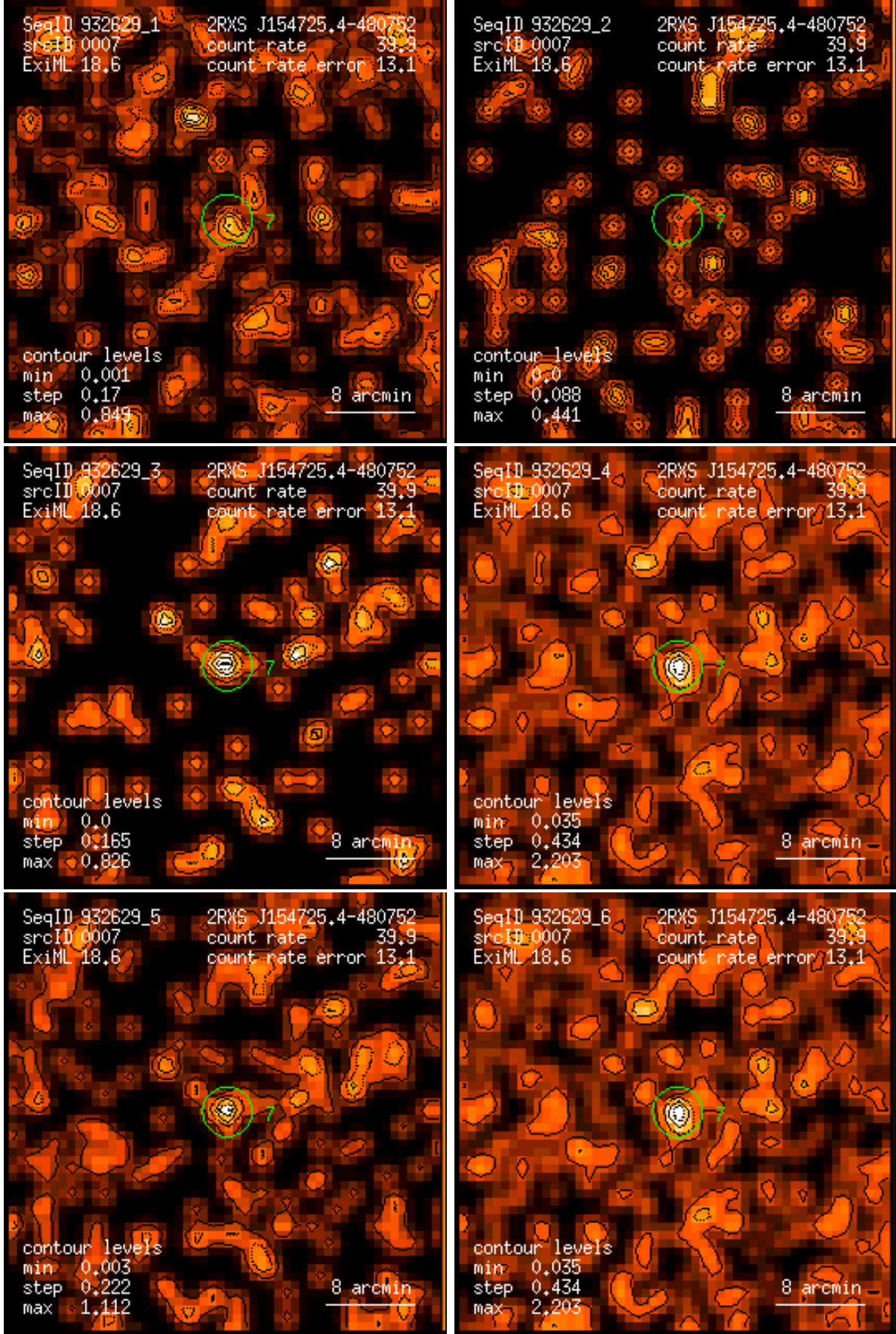
Figure 7: RASS 932629: detection 0007: band rate images, Gaussian filter: (1) PSPC channels 11 – 41, (2) 52 – 90, (3) 91 – 201, (4) 11 – 235, (5) 52 – 201, (6) 11 – 201. Broad band rates in counts/ks. Band rate contour levels in counts/ks/arcmin 2 .
