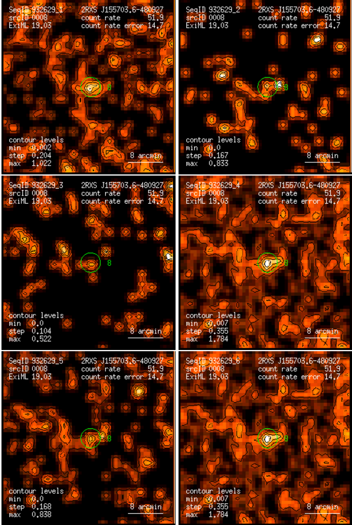
Figure 8: RASS 932629: detection 0008: band rate images, Gaussian filter: (1) PSPC channels 11 – 41, (2) 52 – 90, (3) 91 – 201, (4) 11 – 235, (5) 52 – 201, (6) 11 – 201. Broad band rates in counts/ks. Band rate contour levels in counts/ks/arcmin 2 .
