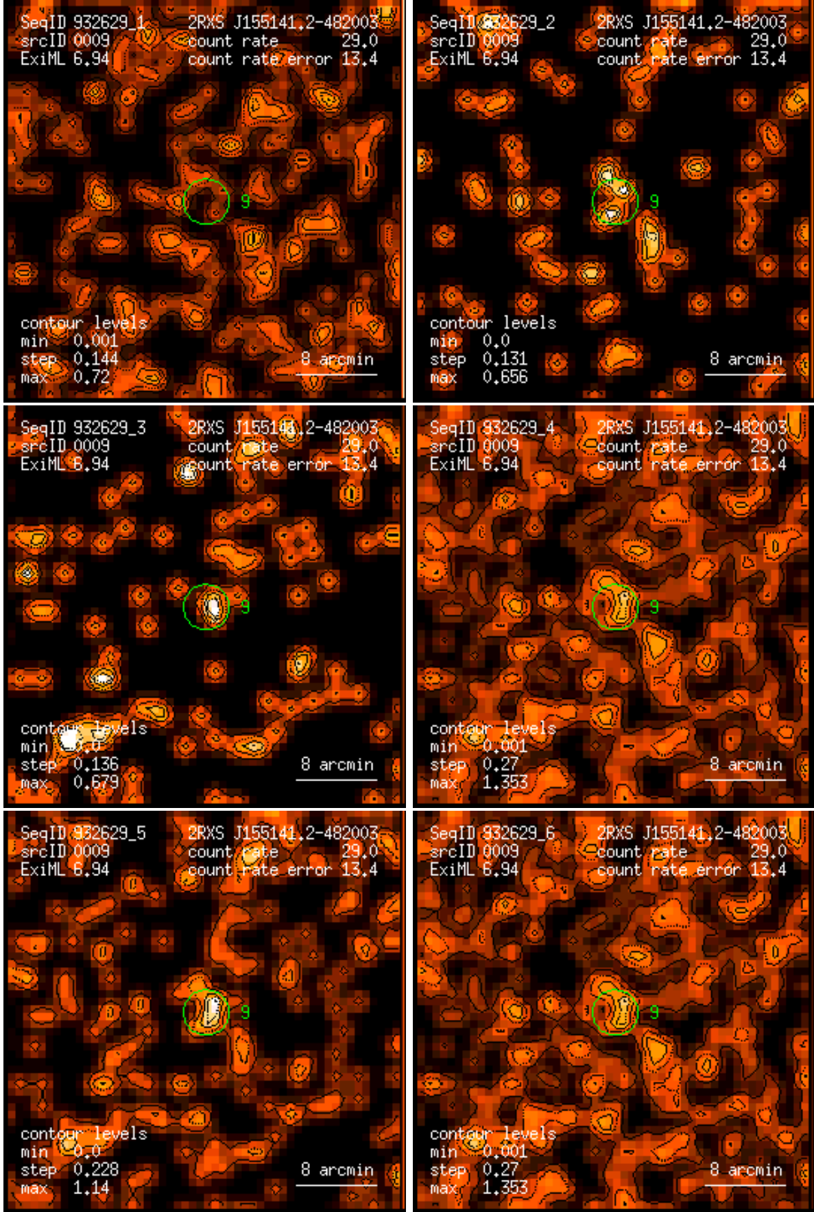
Figure 9: RASS 932629: detection 0009: band rate images, Gaussian filter: (1) PSPC channels 11 – 41, (2) 52 – 90, (3) 91 – 201, (4) 11 – 235, (5) 52 – 201, (6) 11 – 201. Broad band rates in counts/ks. Band rate contour levels in counts/ks/arcmin 2 .
