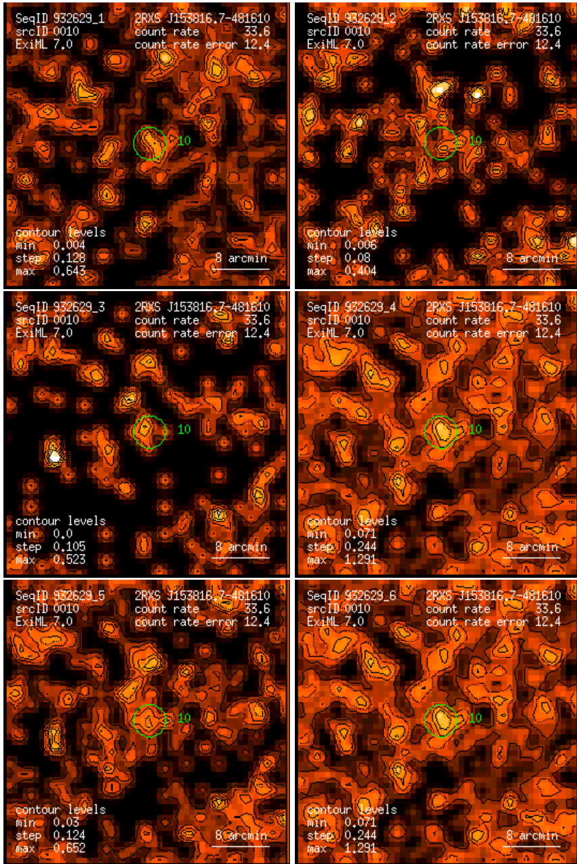
Figure 10: RASS 932629: detection 0010: band rate images, Gaussian filter: (1) PSPC channels 11 – 41, (2) 52 – 90, (3) 91 – 201, (4) 11 – 235, (5) 52 – 201, (6) 11 – 201. Broad band rates in counts/ks. Band rate contour levels in counts/ks/arcmin 2 .
