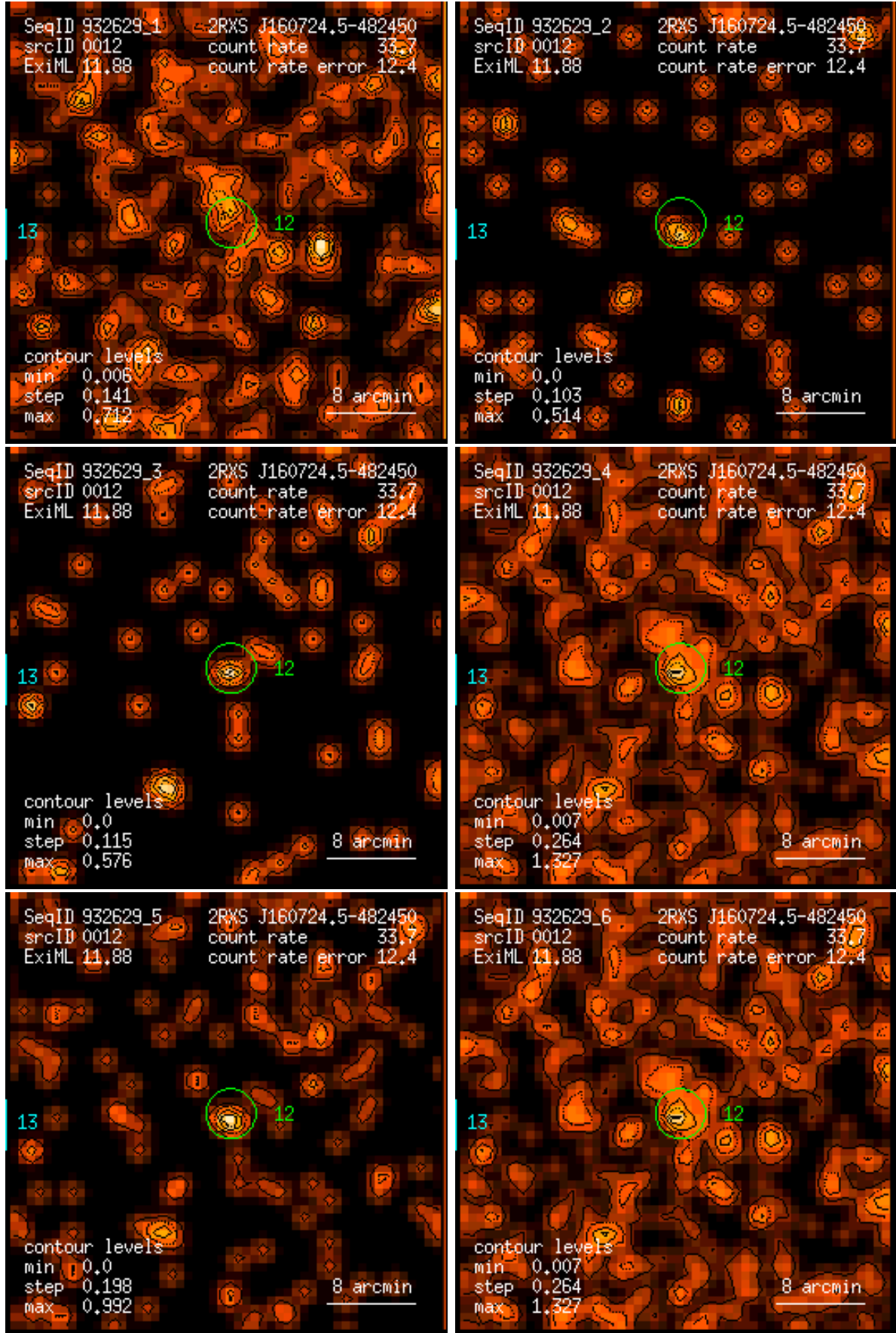
Figure 12: RASS 932629: detection 0012: band rate images, Gaussian filter: (1) PSPC channels 11 – 41, (2) 52 – 90, (3) 91 – 201, (4) 11 – 235, (5) 52 – 201, (6) 11 – 201. Broad band rates in counts/ks. Band rate contour levels in counts/ks/arcmin 2 .
