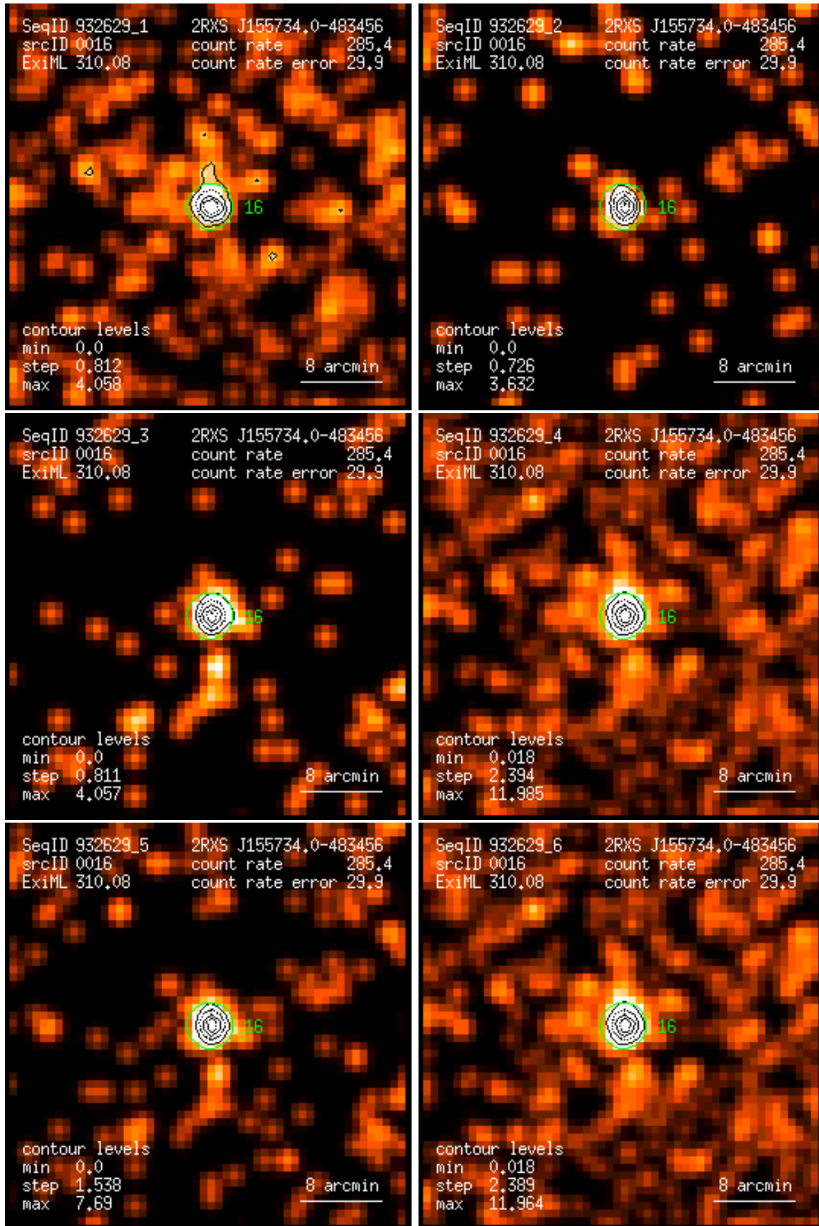
Figure 16: RASS 932629: detection 0016: band rate images, Gaussian filter: (1) PSPC channels 11 – 41, (2) 52 – 90, (3) 91 – 201, (4) 11 – 235, (5) 52 – 201, (6) 11 – 201. Broad band rates in counts/ks. Band rate contour levels in counts/ks/arcmin 2 .
