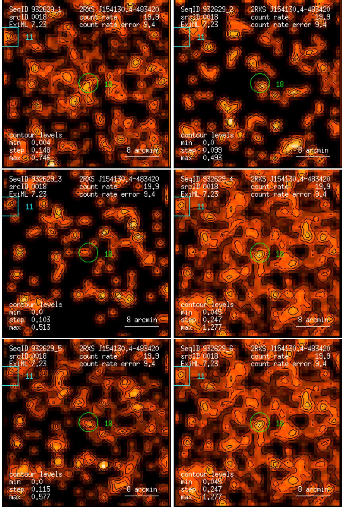
Figure 18: RASS 932629: detection 0018: band rate images, Gaussian filter: (1) PSPC channels 11 – 41, (2) 52 – 90, (3) 91 – 201, (4) 11 – 235, (5) 52 – 201, (6) 11 – 201. Broad band rates in counts/ks. Band rate contour levels in counts/ks/arcmin 2 .
