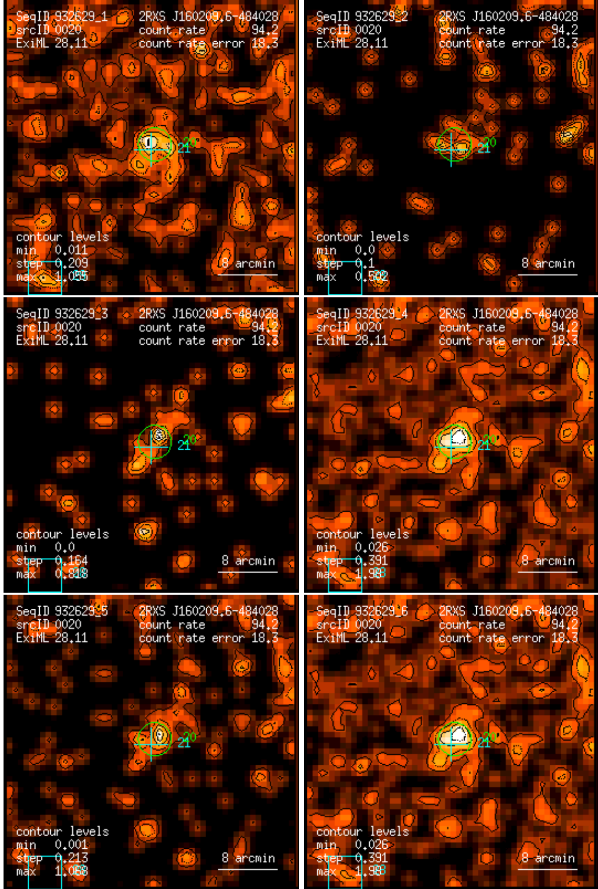
Figure 20: RASS 932629: detection 0020: band rate images, Gaussian filter: (1) PSPC channels 11 – 41, (2) 52 – 90, (3) 91 – 201, (4) 11 – 235, (5) 52 – 201, (6) 11 – 201. Broad band rates in counts/ks. Band rate contour levels in counts/ks/arcmin 2 .
