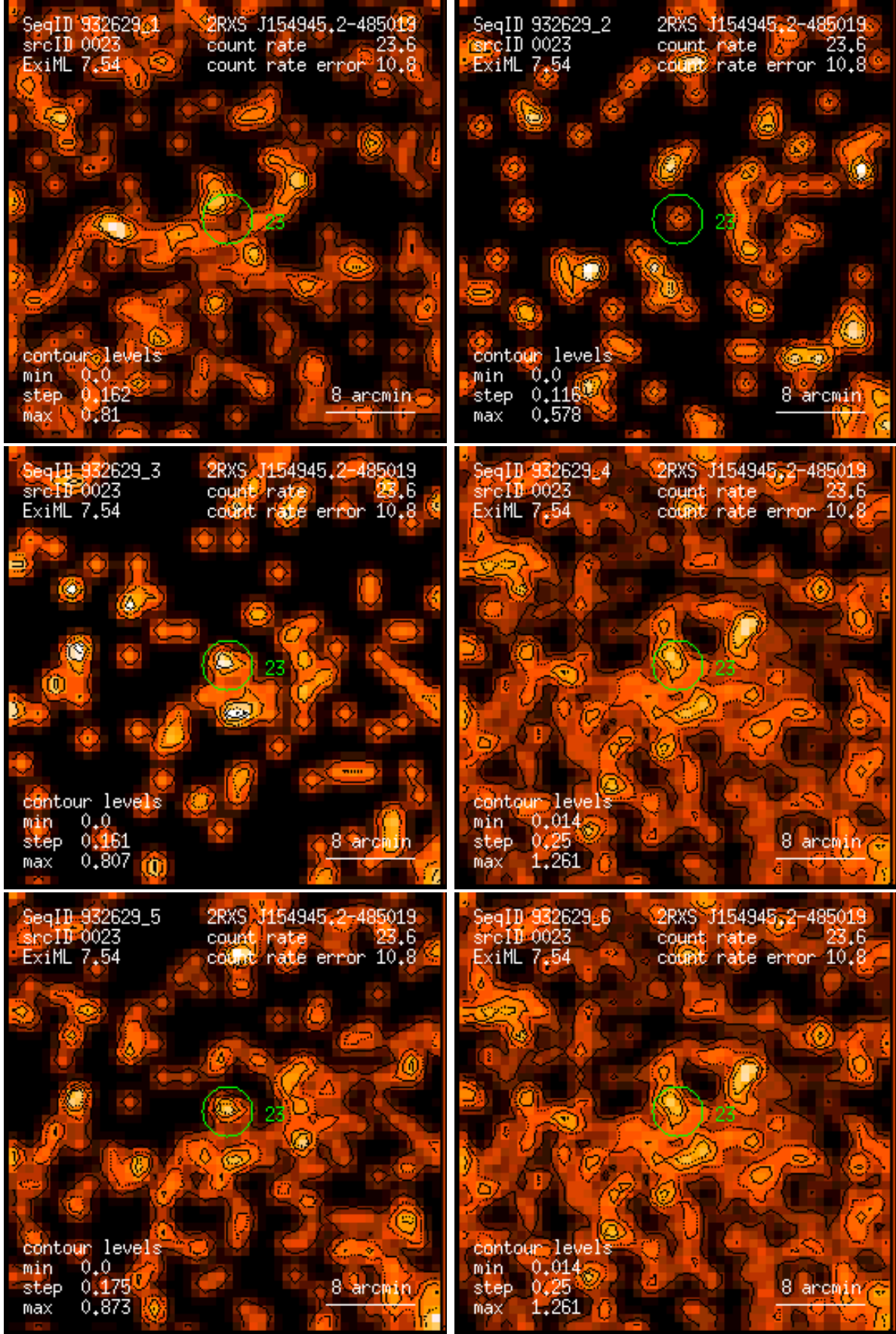
Figure 23: RASS 932629: detection 0023: band rate images, Gaussian filter: (1) PSPC channels 11 – 41, (2) 52 – 90, (3) 91 – 201, (4) 11 – 235, (5) 52 – 201, (6) 11 – 201. Broad band rates in counts/ks. Band rate contour levels in counts/ks/arcmin 2 .
