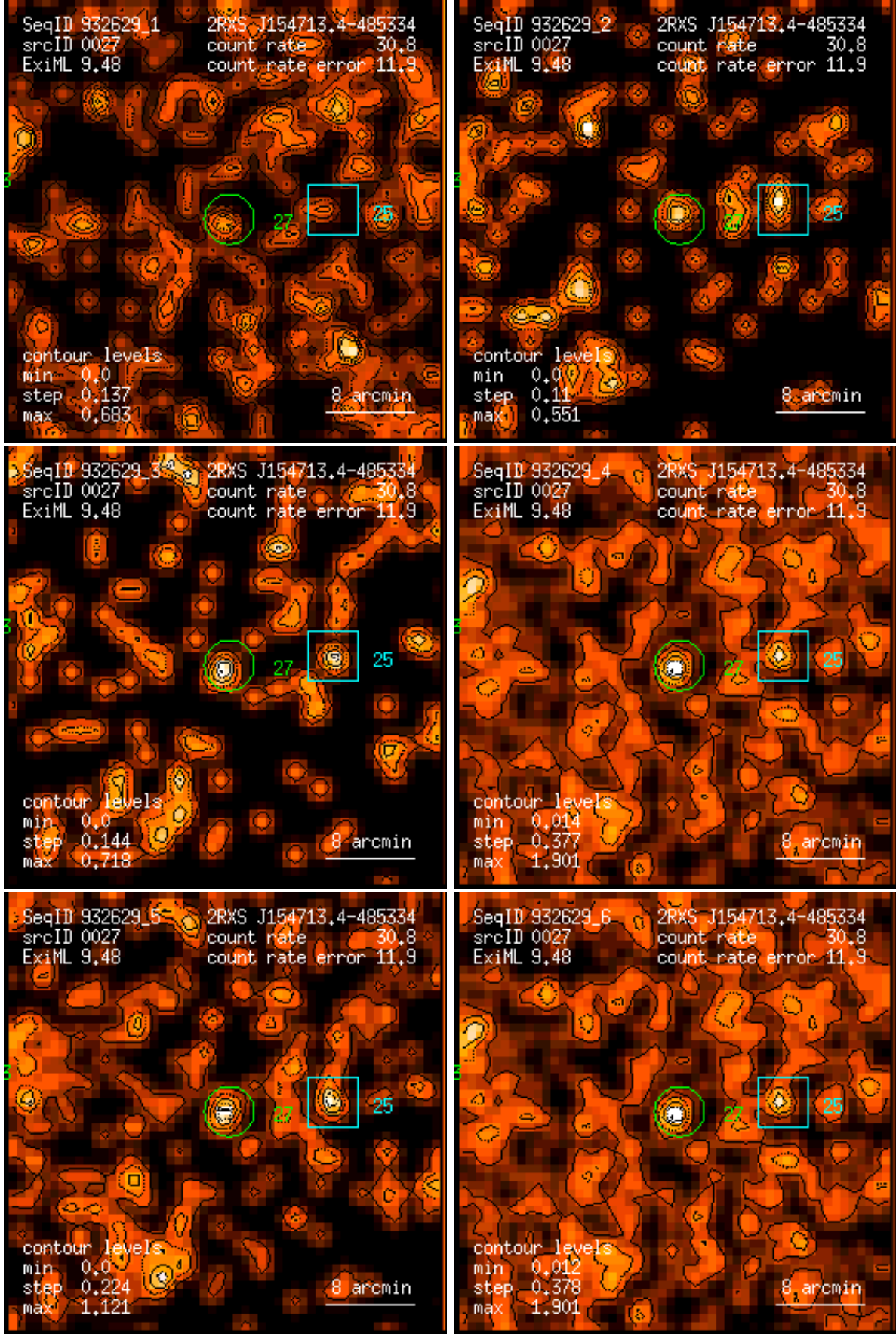
Figure 27: RASS 932629: detection 0027: band rate images, Gaussian filter: (1) PSPC channels 11 – 41, (2) 52 – 90, (3) 91 – 201, (4) 11 – 235, (5) 52 – 201, (6) 11 – 201. Broad band rates in counts/ks. Band rate contour levels in counts/ks/arcmin 2 .
