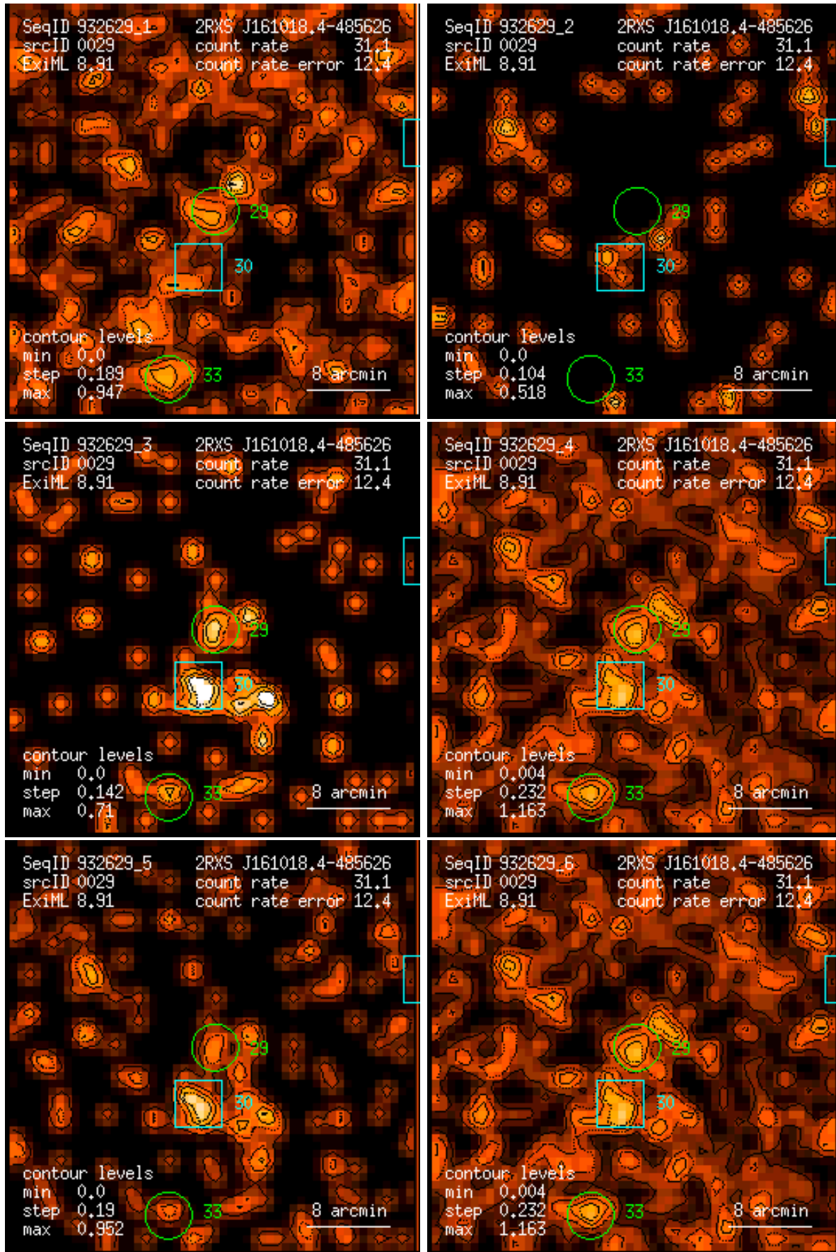
Figure 29: RASS 932629: detection 0029: band rate images, Gaussian filter: (1) PSPC channels 11 – 41, (2) 52 – 90, (3) 91 – 201, (4) 11 – 235, (5) 52 – 201, (6) 11 – 201. Broad band rates in counts/ks. Band rate contour levels in counts/ks/arcmin 2 .
