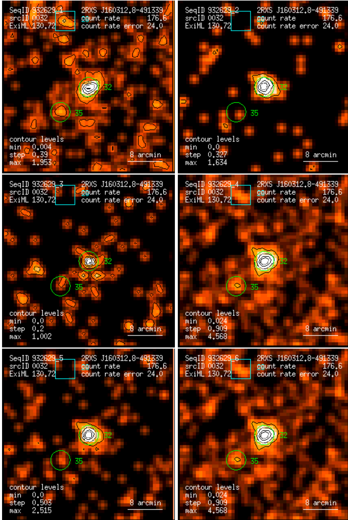
Figure 32: RASS 932629: detection 0032: band rate images, Gaussian filter: (1) PSPC channels 11 – 41, (2) 52 – 90, (3) 91 – 201, (4) 11 – 235, (5) 52 – 201, (6) 11 – 201. Broad band rates in counts/ks. Band rate contour levels in counts/ks/arcmin 2 .
