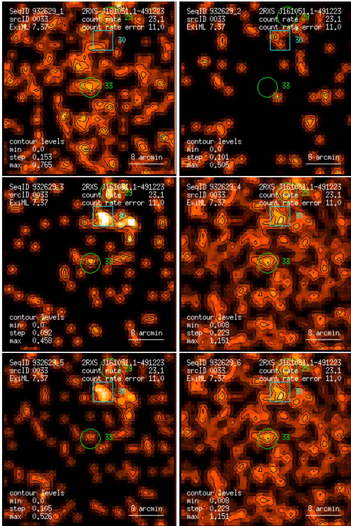
Figure 33: RASS 932629: detection 0033: band rate images, Gaussian filter: (1) PSPC channels 11 – 41, (2) 52 – 90, (3) 91 – 201, (4) 11 – 235, (5) 52 – 201, (6) 11 – 201. Broad band rates in counts/ks. Band rate contour levels in counts/ks/arcmin 2 .
