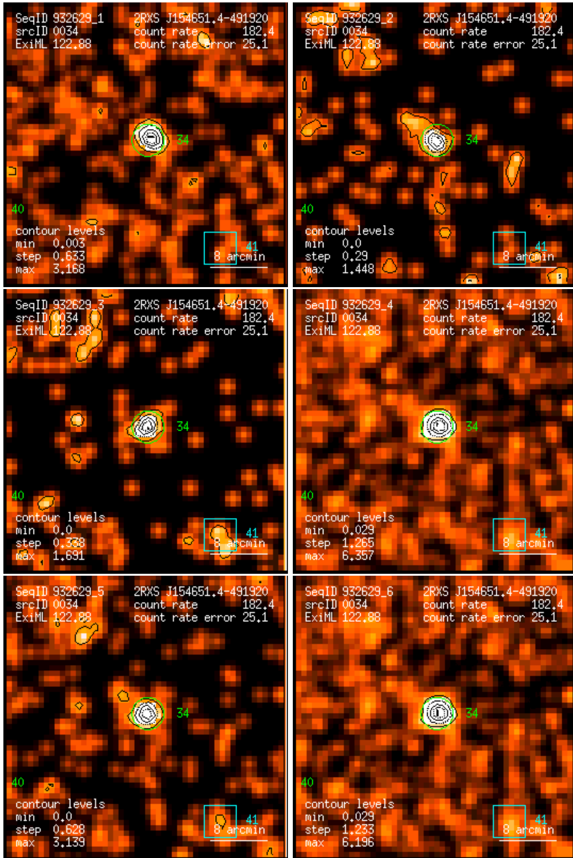
Figure 34: RASS 932629: detection 0034: band rate images, Gaussian filter: (1) PSPC channels 11 – 41, (2) 52 – 90, (3) 91 – 201, (4) 11 – 235, (5) 52 – 201, (6) 11 – 201. Broad band rates in counts/ks. Band rate contour levels in counts/ks/arcmin 2 .
