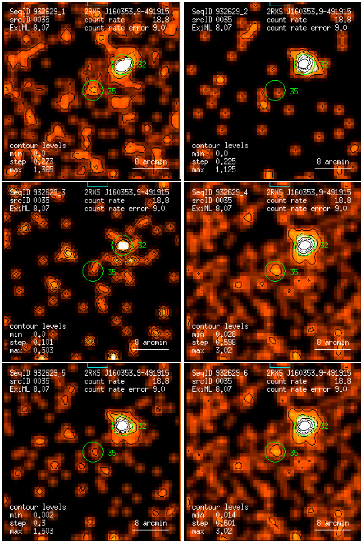
Figure 35: RASS 932629: detection 0035: band rate images, Gaussian filter: (1) PSPC channels 11 – 41, (2) 52 – 90, (3) 91 – 201, (4) 11 – 235, (5) 52 – 201, (6) 11 – 201. Broad band rates in counts/ks. Band rate contour levels in counts/ks/arcmin 2 .
