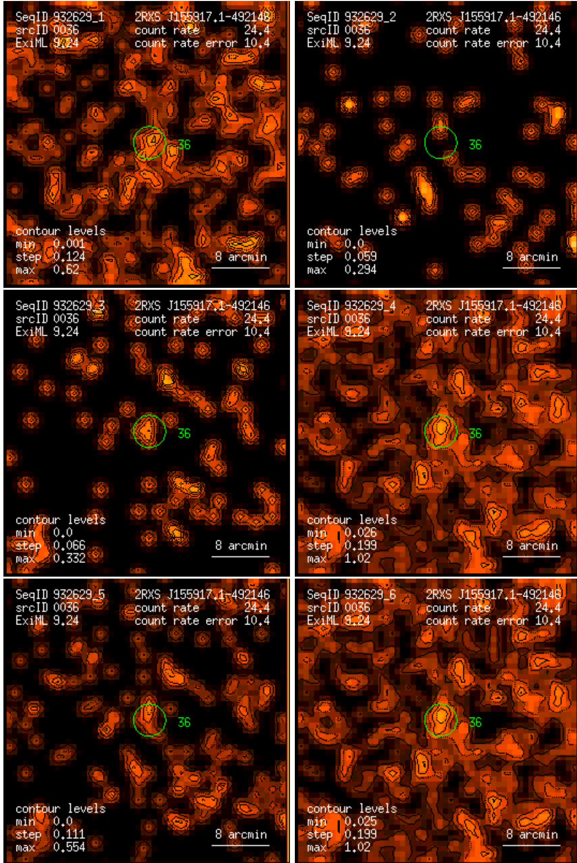
Figure 36: RASS 932629: detection 0036: band rate images, Gaussian filter: (1) PSPC channels 11 – 41, (2) 52 – 90, (3) 91 – 201, (4) 11 – 235, (5) 52 – 201, (6) 11 – 201. Broad band rates in counts/ks. Band rate contour levels in counts/ks/arcmin 2 .
