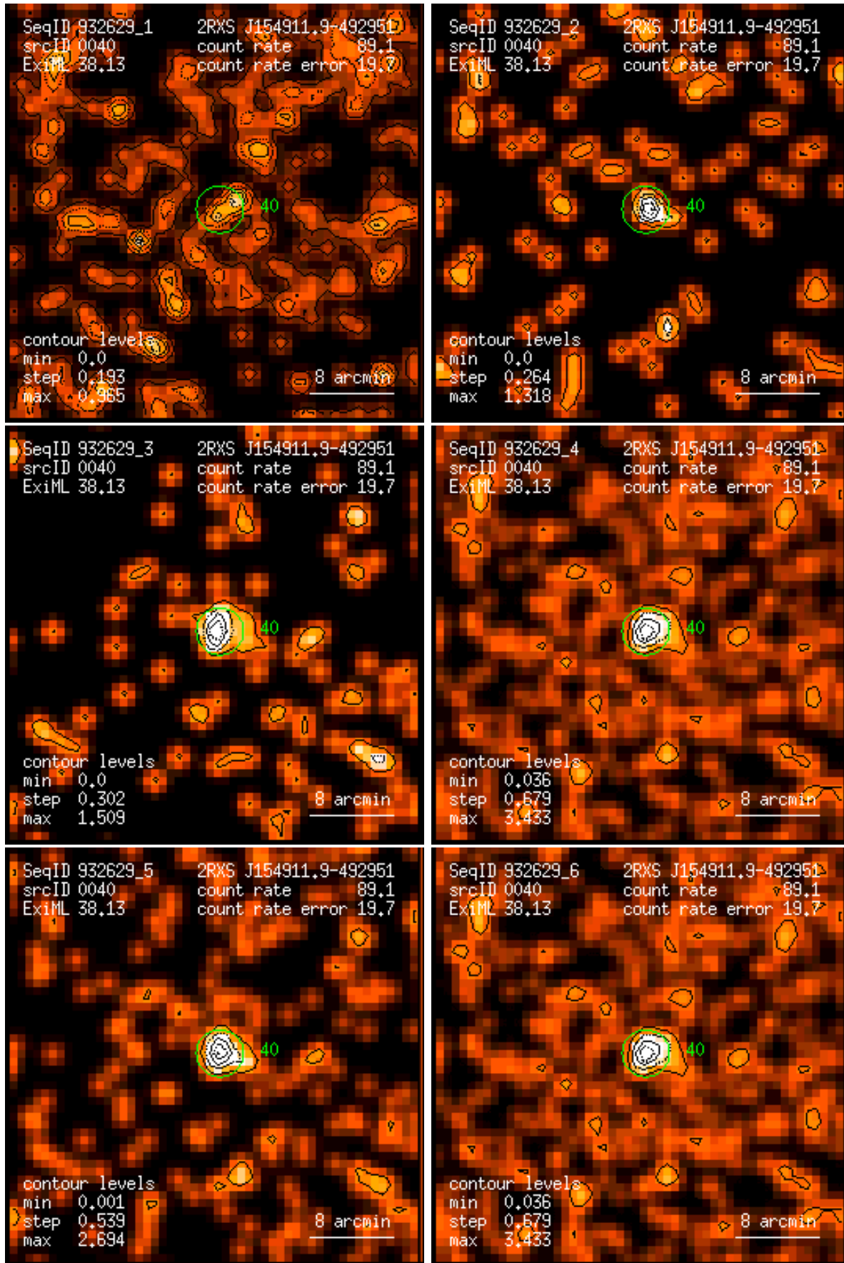
Figure 40: RASS 932629: detection 0040: band rate images, Gaussian filter: (1) PSPC channels 11 – 41, (2) 52 – 90, (3) 91 – 201, (4) 11 – 235, (5) 52 – 201, (6) 11 – 201. Broad band rates in counts/ks. Band rate contour levels in counts/ks/arcmin 2 .
