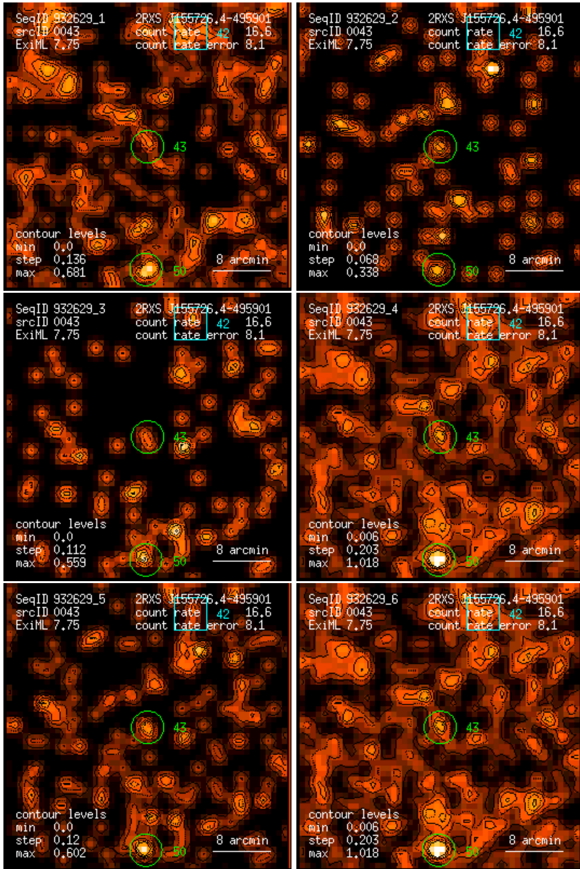
Figure 43: RASS 932629: detection 0043: band rate images, Gaussian filter: (1) PSPC channels 11 – 41, (2) 52 – 90, (3) 91 – 201, (4) 11 – 235, (5) 52 – 201, (6) 11 – 201. Broad band rates in counts/ks. Band rate contour levels in counts/ks/arcmin 2 .
