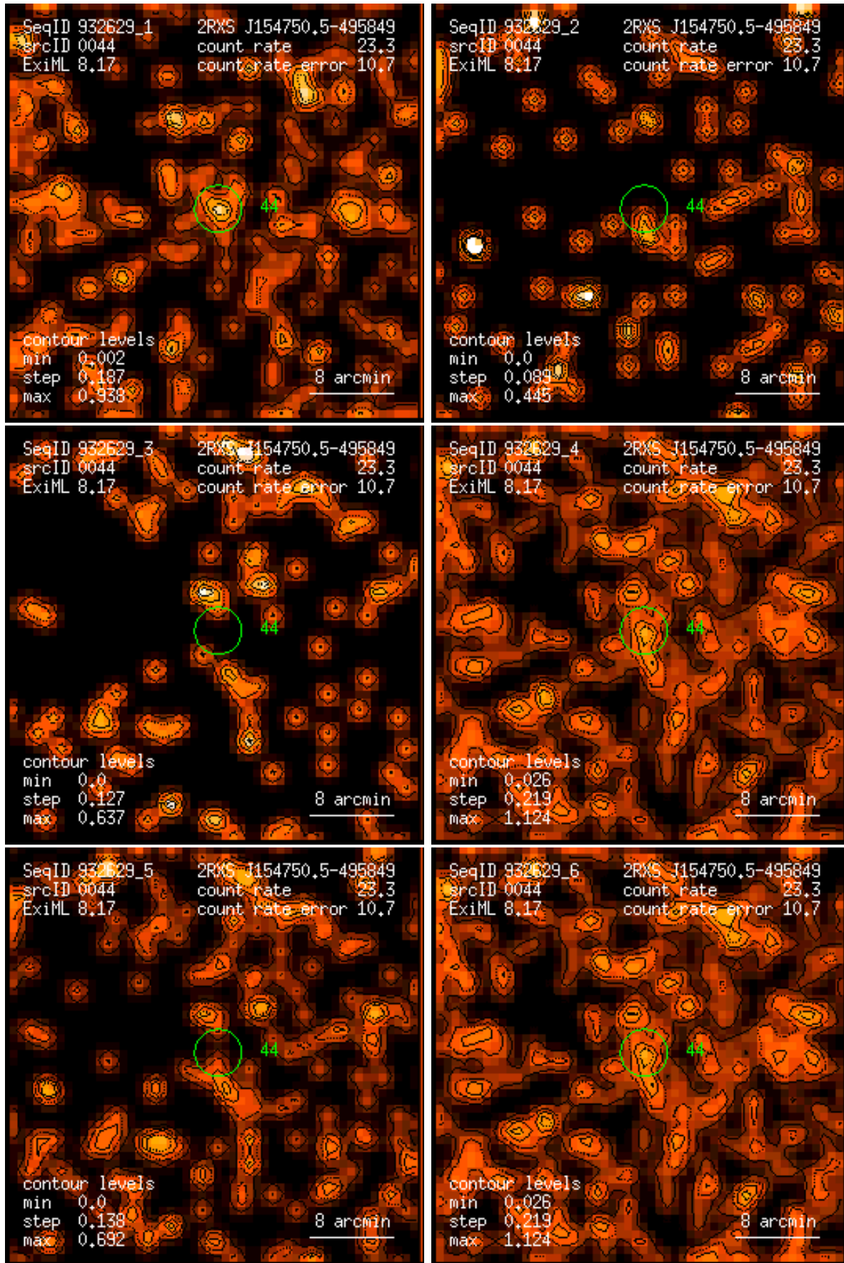
Figure 44: RASS 932629: detection 0044: band rate images, Gaussian filter: (1) PSPC channels 11 – 41, (2) 52 – 90, (3) 91 – 201, (4) 11 – 235, (5) 52 – 201, (6) 11 – 201. Broad band rates in counts/ks. Band rate contour levels in counts/ks/arcmin 2 .
