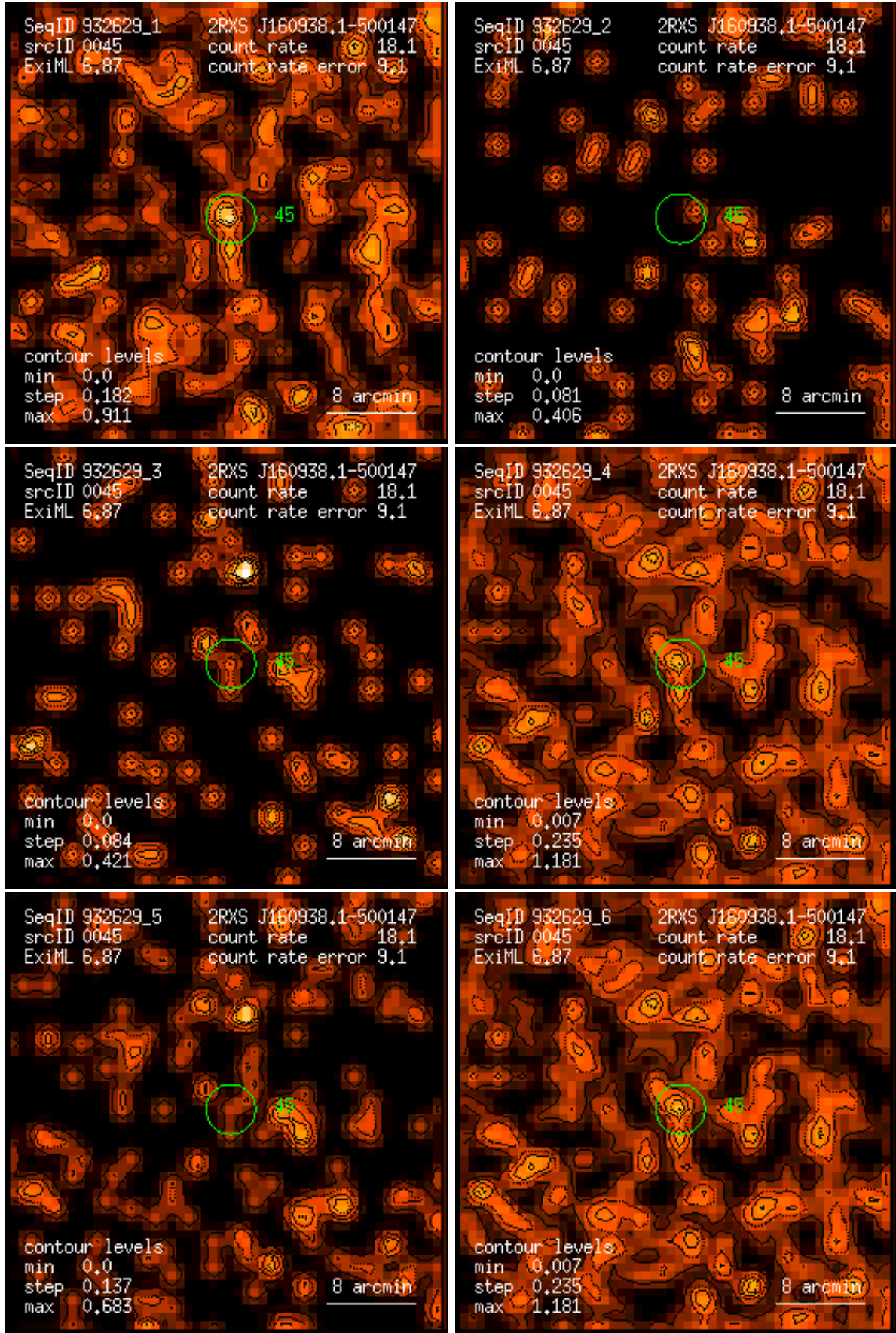
Figure 45: RASS 932629: detection 0045: band rate images, Gaussian filter: (1) PSPC channels 11 – 41, (2) 52 – 90, (3) 91 – 201, (4) 11 – 235, (5) 52 – 201, (6) 11 – 201. Broad band rates in counts/ks. Band rate contour levels in counts/ks/arcmin 2 .
