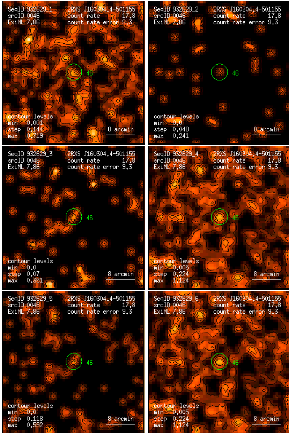
Figure 46: RASS 932629: detection 0046: band rate images, Gaussian filter: (1) PSPC channels 11 – 41, (2) 52 – 90, (3) 91 – 201, (4) 11 – 235, (5) 52 – 201, (6) 11 – 201. Broad band rates in counts/ks. Band rate contour levels in counts/ks/arcmin 2 .
