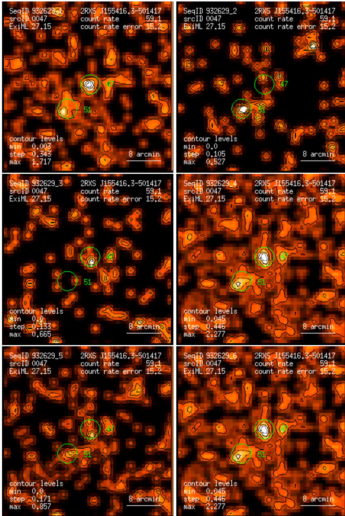
Figure 47: RASS 932629: detection 0047: band rate images, Gaussian filter: (1) PSPC channels 11 – 41, (2) 52 – 90, (3) 91 – 201, (4) 11 – 235, (5) 52 – 201, (6) 11 – 201. Broad band rates in counts/ks. Band rate contour levels in counts/ks/arcmin 2 .
