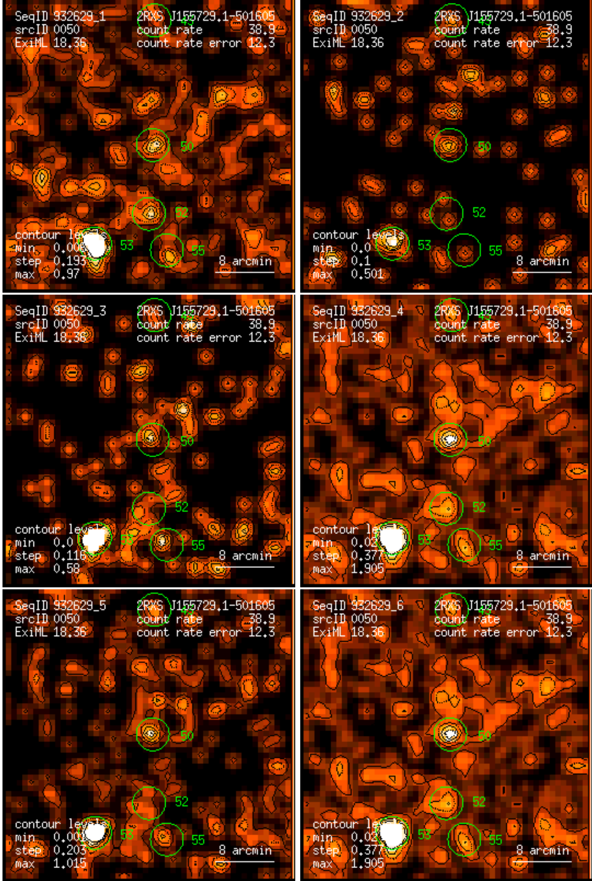
Figure 50: RASS 932629: detection 0050: band rate images, Gaussian filter: (1) PSPC channels 11 – 41, (2) 52 – 90, (3) 91 – 201, (4) 11 – 235, (5) 52 – 201, (6) 11 – 201. Broad band rates in counts/ks. Band rate contour levels in counts/ks/arcmin 2 .
