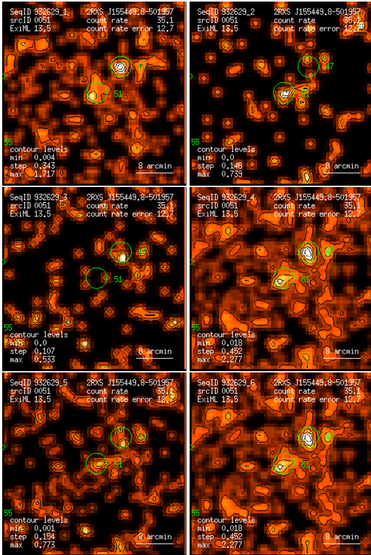
Figure 51: RASS 932629: detection 0051: band rate images, Gaussian filter: (1) PSPC channels 11 – 41, (2) 52 – 90, (3) 91 – 201, (4) 11 – 235, (5) 52 – 201, (6) 11 – 201. Broad band rates in counts/ks. Band rate contour levels in counts/ks/arcmin 2 .
