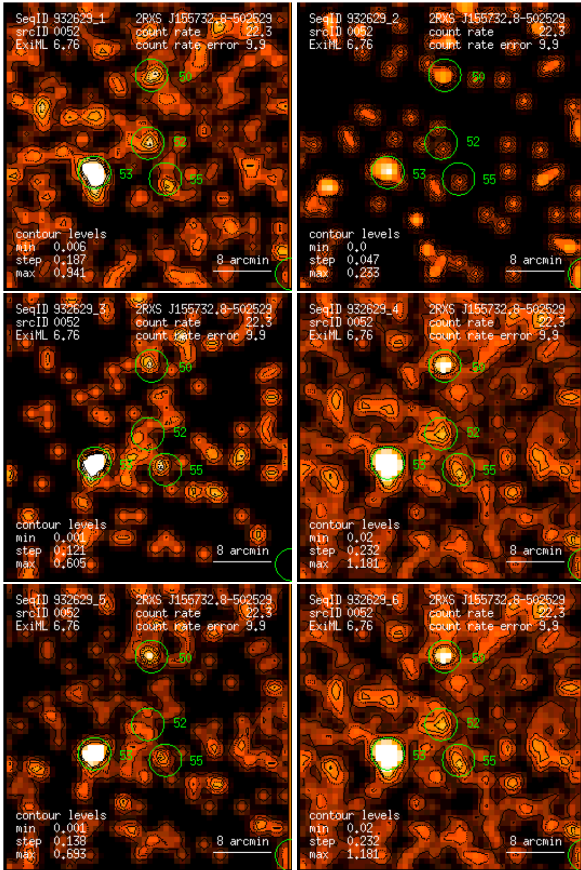
Figure 52: RASS 932629: detection 0052: band rate images, Gaussian filter: (1) PSPC channels 11 – 41, (2) 52 – 90, (3) 91 – 201, (4) 11 – 235, (5) 52 – 201, (6) 11 – 201. Broad band rates in counts/ks. Band rate contour levels in counts/ks/arcmin 2 .
