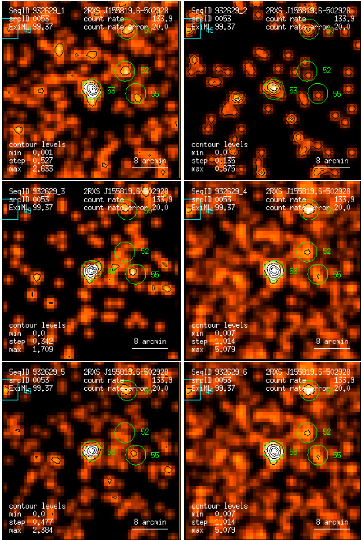
Figure 53: RASS 932629: detection 0053: band rate images, Gaussian filter: (1) PSPC channels 11 – 41, (2) 52 – 90, (3) 91 – 201, (4) 11 – 235, (5) 52 – 201, (6) 11 – 201. Broad band rates in counts/ks. Band rate contour levels in counts/ks/arcmin 2 .
