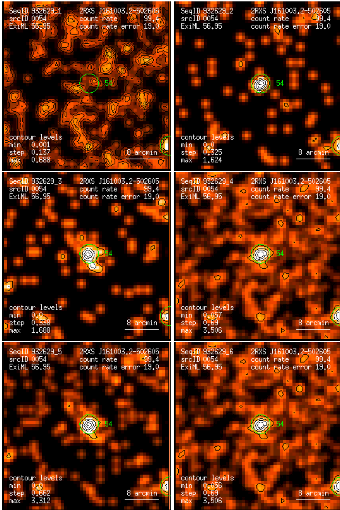
Figure 54: RASS 932629: detection 0054: band rate images, Gaussian filter: (1) PSPC channels 11 – 41, (2) 52 – 90, (3) 91 – 201, (4) 11 – 235, (5) 52 – 201, (6) 11 – 201. Broad band rates in counts/ks. Band rate contour levels in counts/ks/arcmin 2 .
