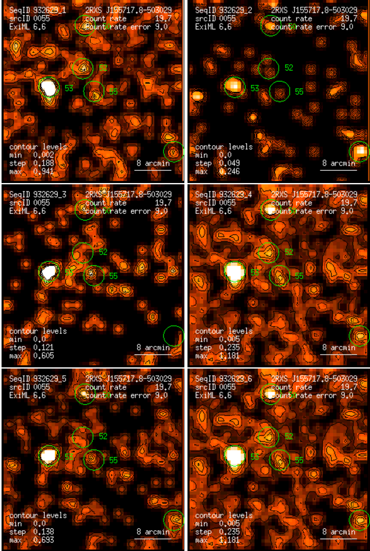
Figure 55: RASS 932629: detection 0055: band rate images, Gaussian filter: (1) PSPC channels 11 – 41, (2) 52 – 90, (3) 91 – 201, (4) 11 – 235, (5) 52 – 201, (6) 11 – 201. Broad band rates in counts/ks. Band rate contour levels in counts/ks/arcmin 2 .
