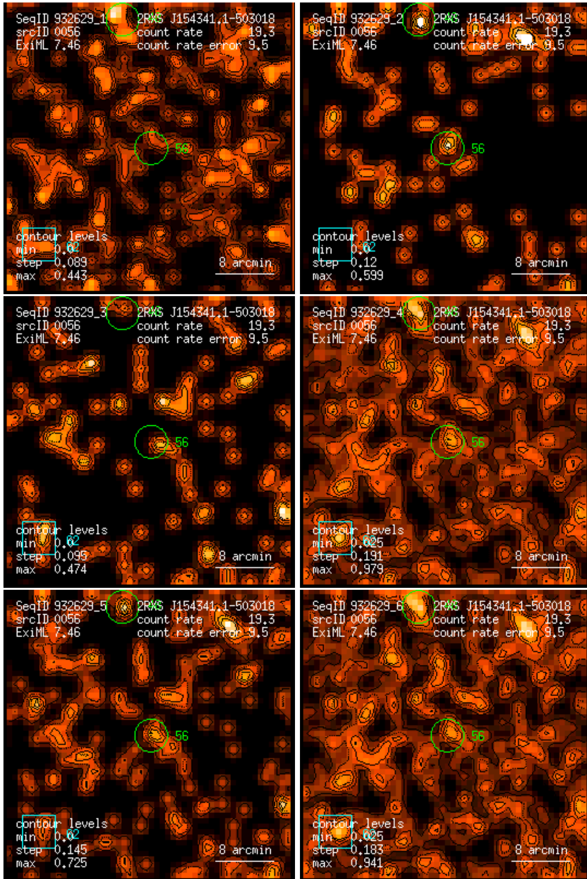
Figure 56: RASS 932629: detection 0056: band rate images, Gaussian filter: (1) PSPC channels 11 – 41, (2) 52 – 90, (3) 91 – 201, (4) 11 – 235, (5) 52 – 201, (6) 11 – 201. Broad band rates in counts/ks. Band rate contour levels in counts/ks/arcmin 2 .
