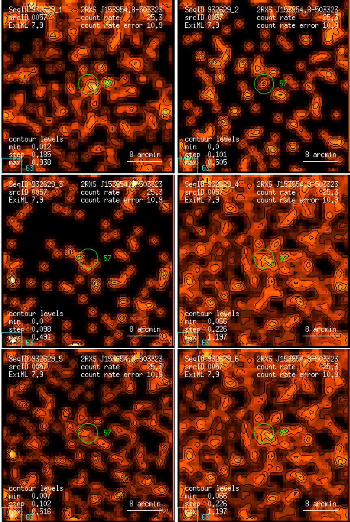
Figure 57: RASS 932629: detection 0057: band rate images, Gaussian filter: (1) PSPC channels 11 – 41, (2) 52 – 90, (3) 91 – 201, (4) 11 – 235, (5) 52 – 201, (6) 11 – 201. Broad band rates in counts/ks. Band rate contour levels in counts/ks/arcmin 2 .
