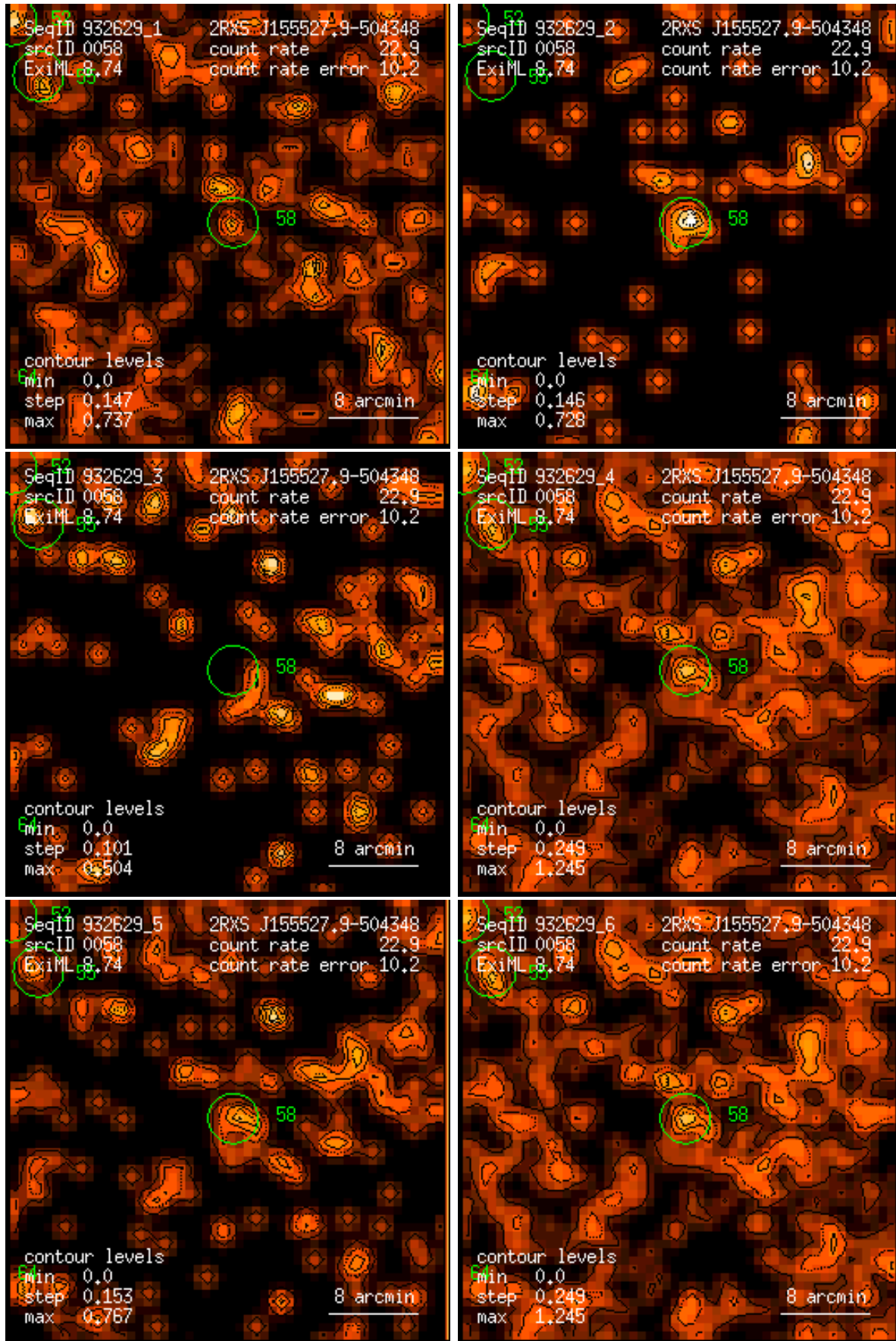
Figure 58: RASS 932629: detection 0058: band rate images, Gaussian filter: (1) PSPC channels 11 – 41, (2) 52 – 90, (3) 91 – 201, (4) 11 – 235, (5) 52 – 201, (6) 11 – 201. Broad band rates in counts/ks. Band rate contour levels in counts/ks/arcmin 2 .
