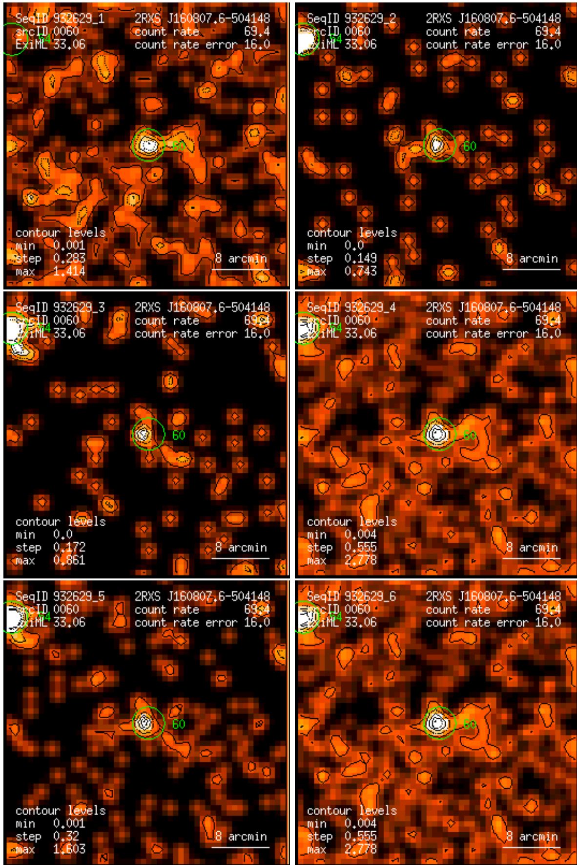
Figure 60: RASS 932629: detection 0060: band rate images, Gaussian filter: (1) PSPC channels 11 – 41, (2) 52 – 90, (3) 91 – 201, (4) 11 – 235, (5) 52 – 201, (6) 11 – 201. Broad band rates in counts/ks. Band rate contour levels in counts/ks/arcmin 2 .
